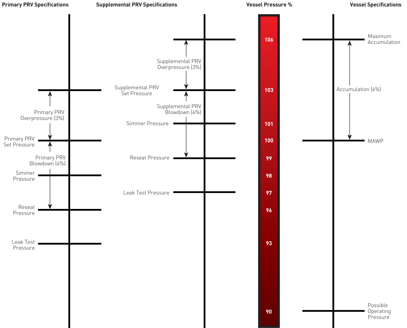
FIGURE 3-2 Typical Section I Multiple PRV Installation
