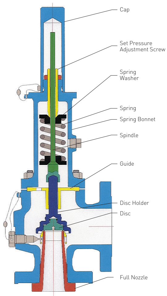
FIGURE 4-14 API 526 Direct Spring PRV
