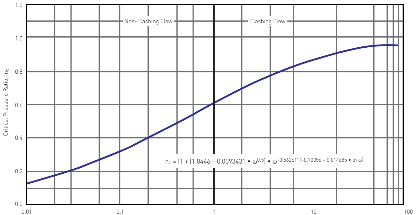
FIGURE 6-2 Omega Parameter, \omega Critical Pressure Ratio for Two-Phase Flow
