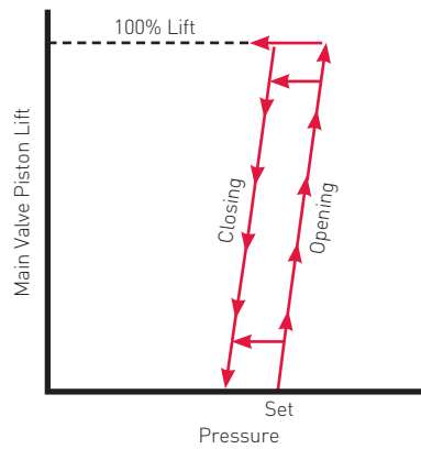
FIGURE 4-34 Main Valve Lift vs Set Pressure for Modulating Action Pilot Operated PRV
