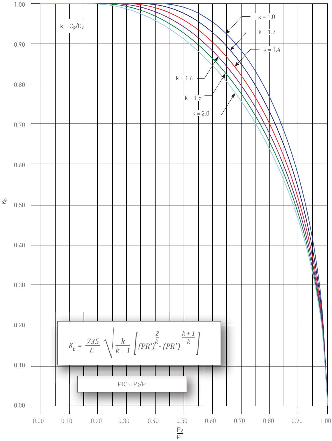
FIGURE 7-22 Anderson Greenwood Series 90/9000 - POPRV Back Pressure Correction Factor ( K_b ) - Gas Service
