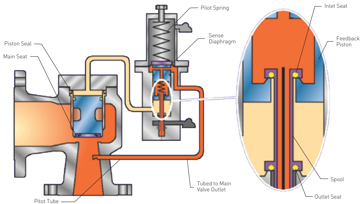
FIGURE 4-32 Modulating Action Pilot Operated PRV (open)
