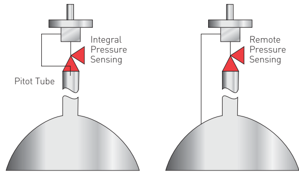
FIGURE 4-36 Remote Sense Pilot Operated PRV
