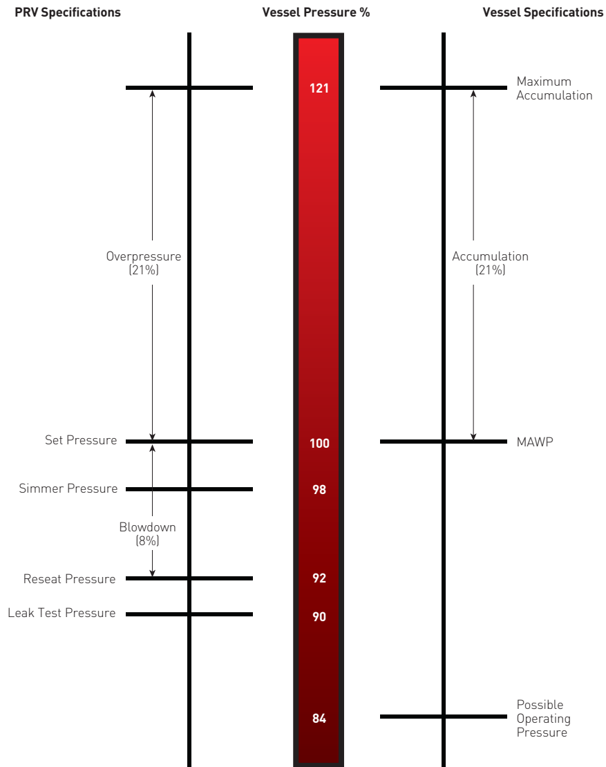
FIGURE 3-9 Typical Section VIII Single Device Installation (Fire) - Set at the MAWP of the Vessel
