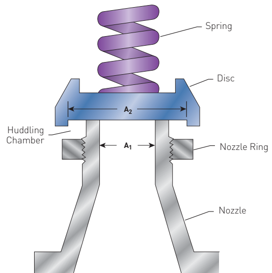
FIGURE 4-5 Generic Direct Spring PRV Trim
