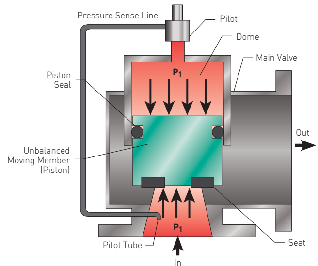
FIGURE 4-25 Piston Type Pilot Operated PRV
