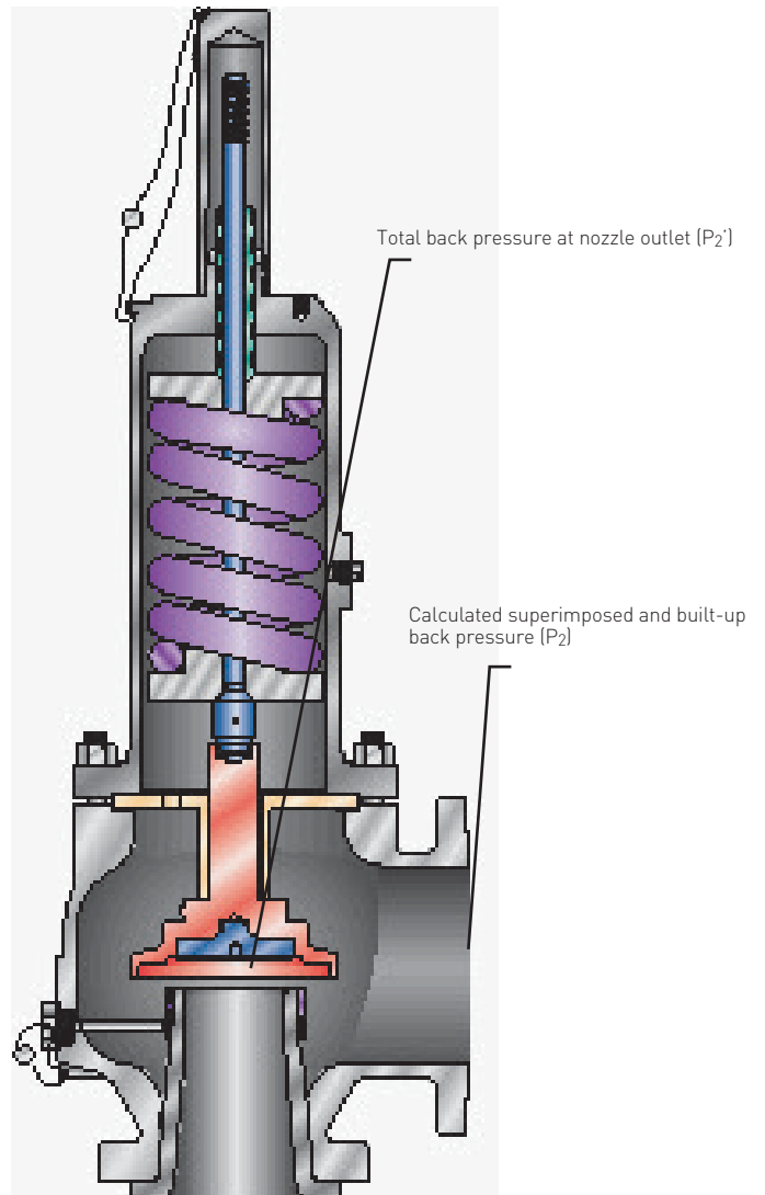
FIGURE 8-3 Relationship of P_2' and P_2
