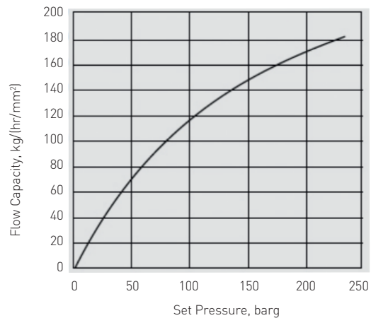
FIGURE 6-4 ASME Section VIII Appendix 11 Available Mass Flux - Saturated Water
