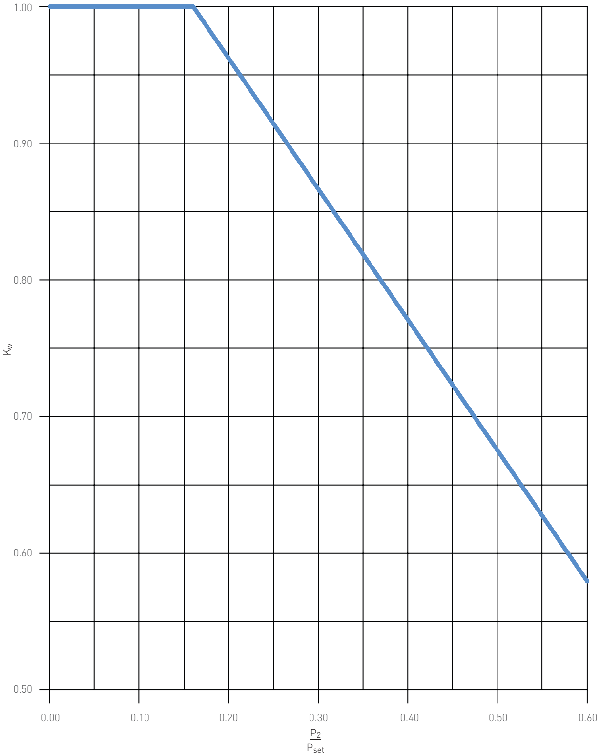
FIGURE 8-11 Crosby Series JLT-JBS-E Balanced Bellows Direct Spring PRV Back Pressure Correction Factor ( K_w ) - Liquid Service
