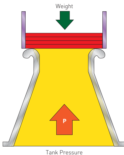
FIGURE 4-1 Weight Loaded Pressure Relief Valve
