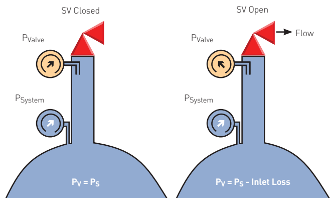
FIGURE 4-18 Inlet Piping Effects on Direct Acting PRV
