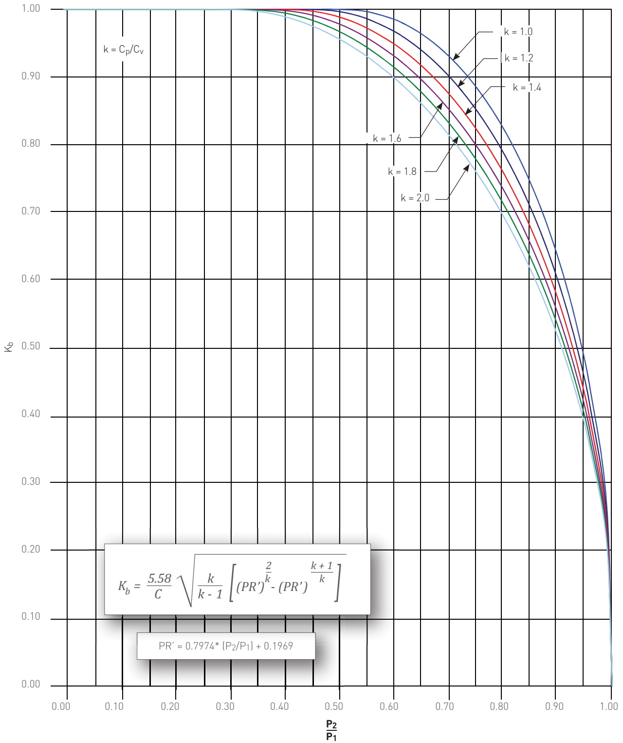
FIGURE 8-21 Anderson Greenwood Series 81P (-8 Orifice Only) Balanced Piston Direct Spring PRV Back Pressure Correction Factor ( K_b ) - Gas Service
