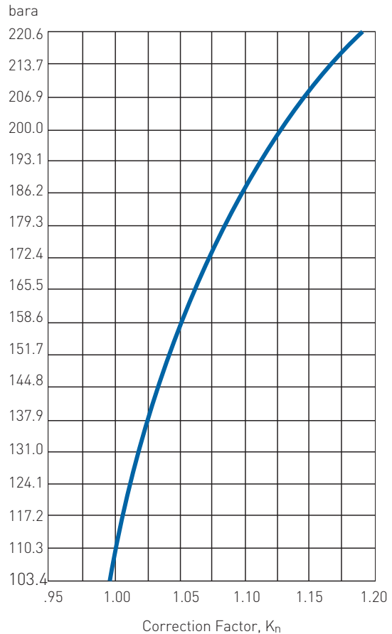
FIGURE 8-28 Correction Factor for High Pressure Steam, K_n
