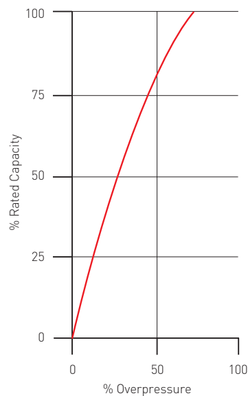
FIGURE 4-3 Typical Weight Loaded Pressure/Vacuum Vent Capacity vs Overpressure Characteristic
