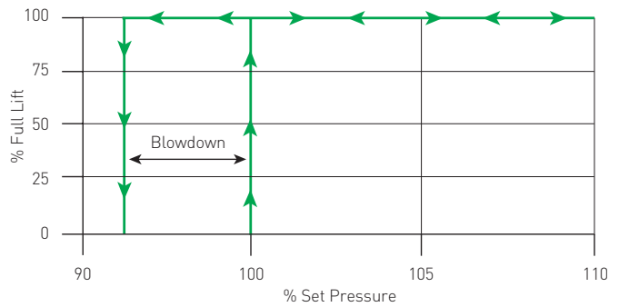
FIGURE 4-30 Main Valve Lift vs Set Pressure for Pop Action Pilot Operated PRV
