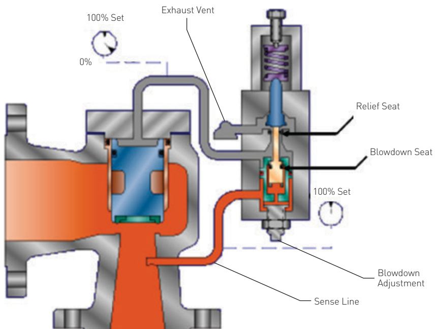
FIGURE 4-29 Pop Action Pilot Operated PRV (open)
