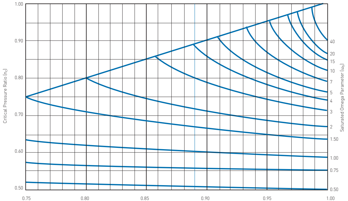
FIGURE 6-3 Saturated Pressure Ratio ( h_s ) Critical Pressure Ratio for Low Subcooled Region Flashing Liquids
