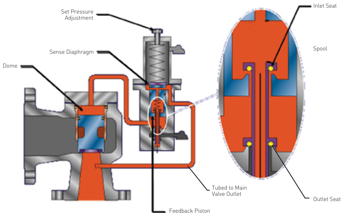
FIGURE 4-31 Modulating Action Pilot Operated PRV (closed)
