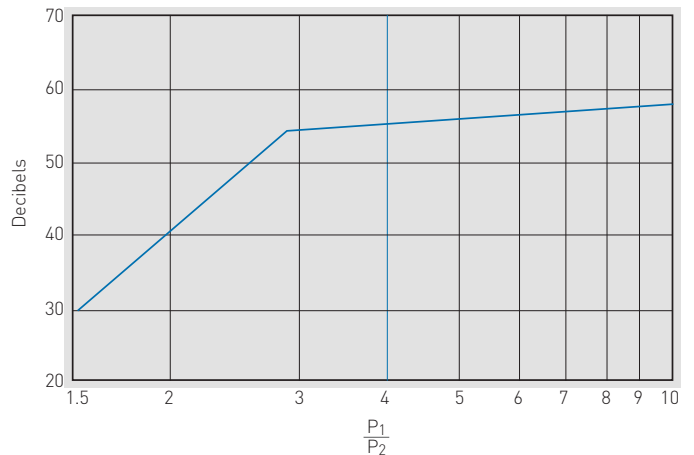
FIGURE 5-6 Sound Pressure Level at 100 Feet from Point of Discharge
