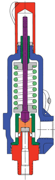
FIGURE 4-18 Inlet Piping Effects on Direct Acting PRV
