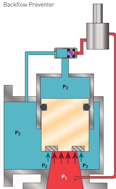
FIGURE 4-40 Backflow Preventer
