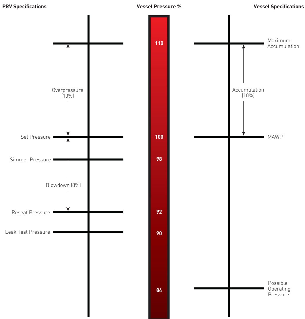
FIGURE 3-7 Typical Section VIII Single Device Installation (Non-Fire) - Set at the MAWP of the Vessel
