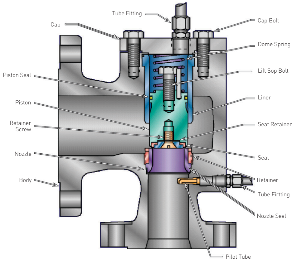
FIGURE 4-35 Piston Type Main Valve Components
