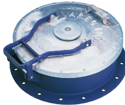
FIGURE 4-4 Emergency Pressure Relief Device
