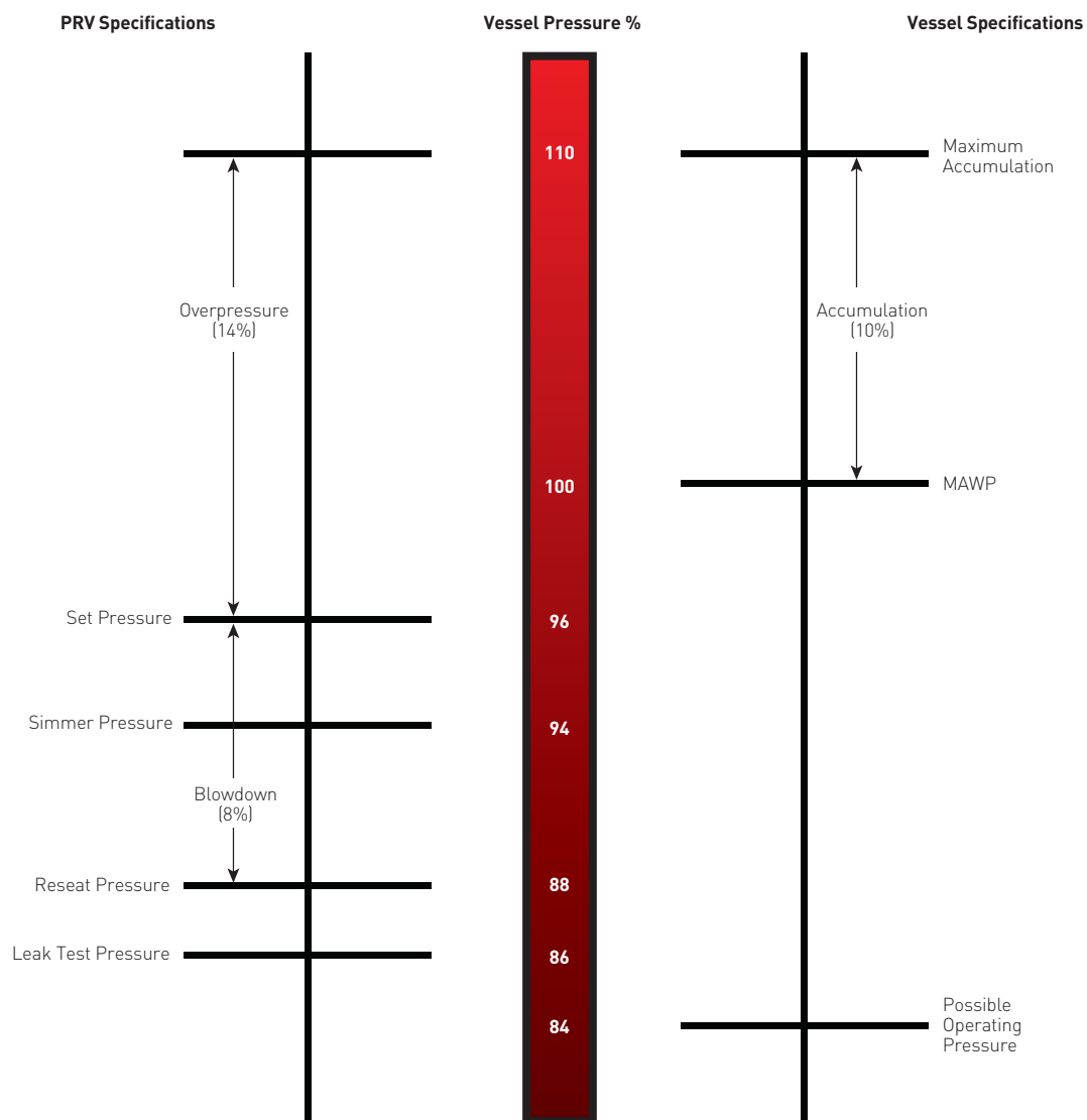
FIGURE 3-8 Typical Section VIII Single Device Installation (Non-Fire) - Set below the MAWP of the Vessel
