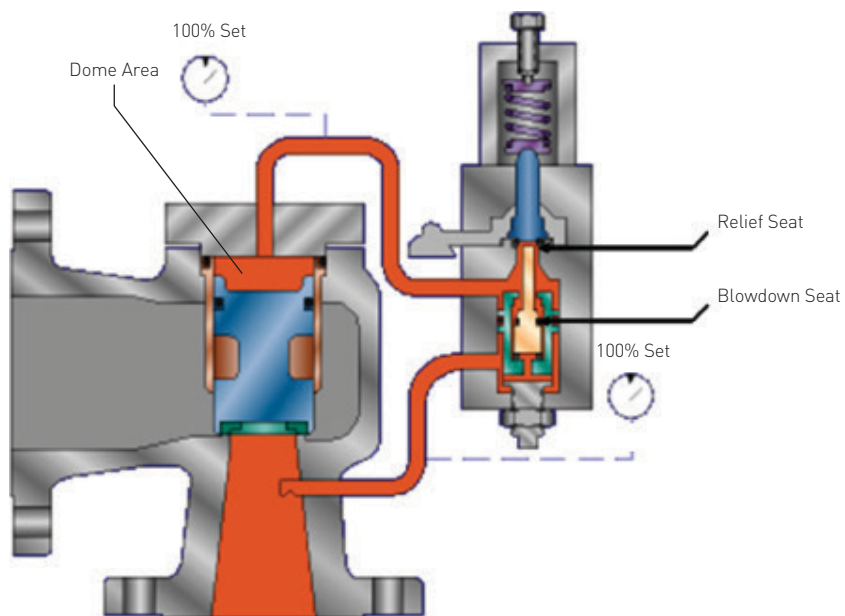
FIGURE 4-28 Pop Action Pilot Operated PRV (closed)
