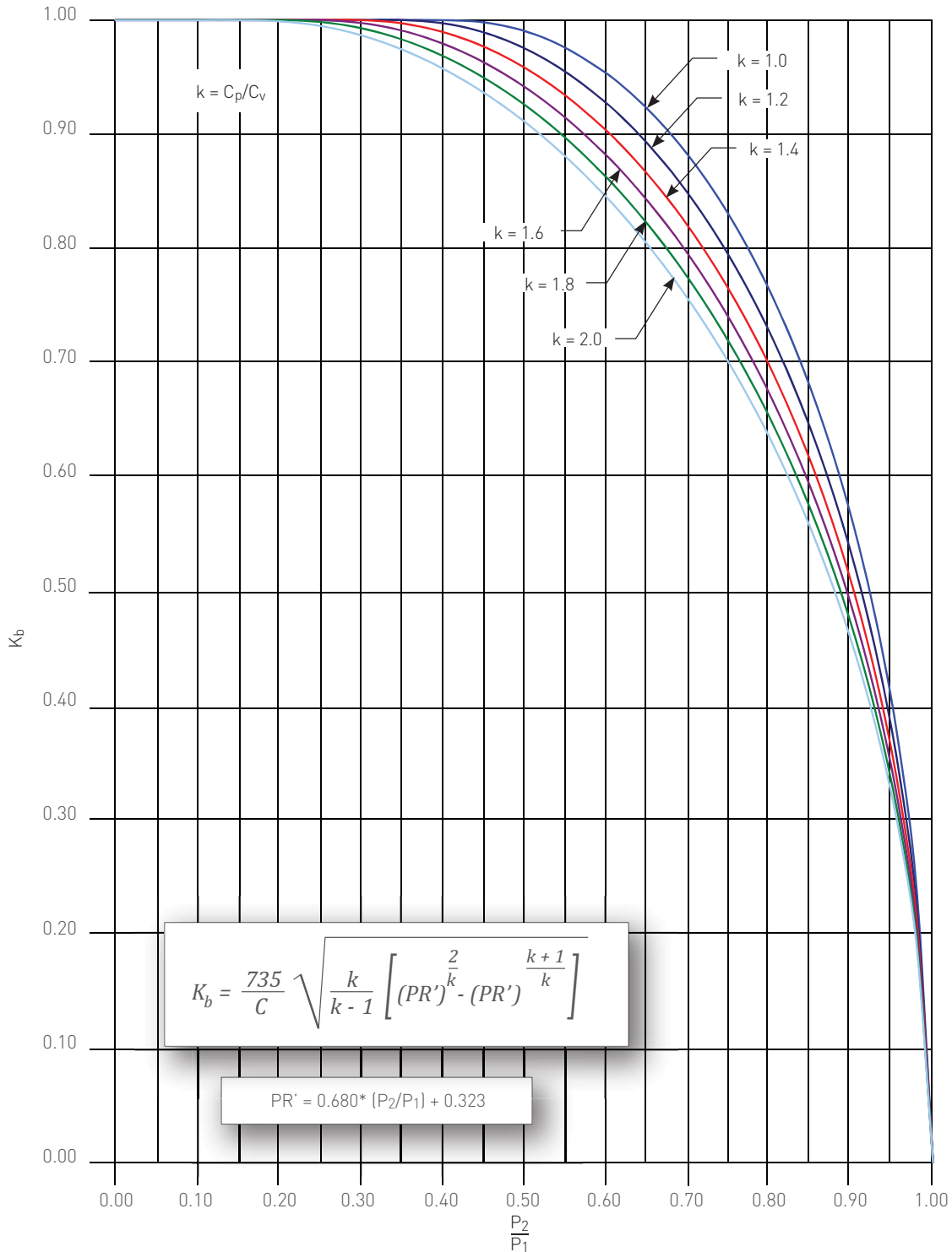
FIGURE 7-26 Anderson Greenwood Series LCP Pilot Operated PRV Back Pressure Correction Factor ( K_b ) - Gas Service
