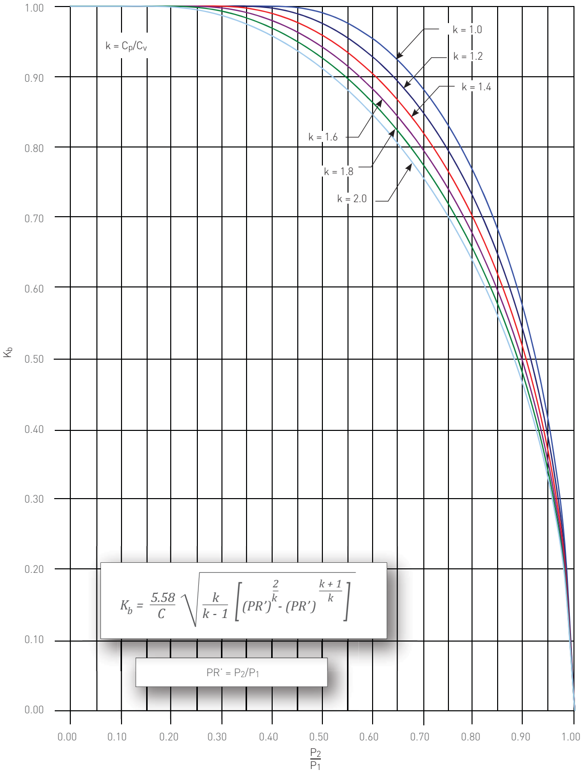
FIGURE 8-22 Anderson Greenwood Series 90/9000 - POPRV Back Pressure Correction Factor ( K_b ) - Gas Service
