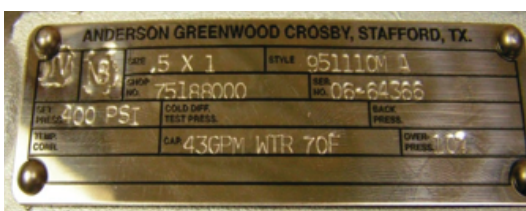
FIGURE 3-12 Typical ASME Section VIII Nameplate
