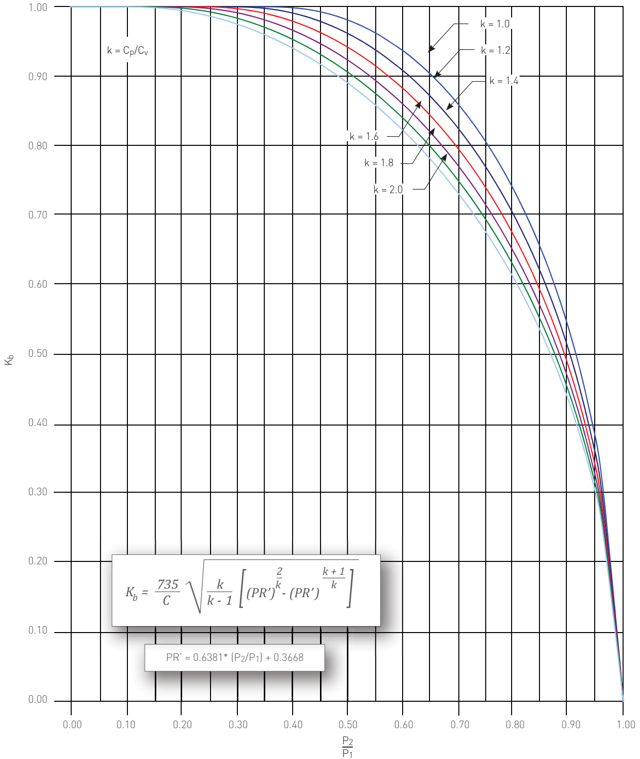
FIGURE 7-18 Anderson Greenwood Series 63B (-7 Orifice Only) Conventional Direct Acting PRV Back Pressure Correction Factor ( K_b ) - Gas Service
