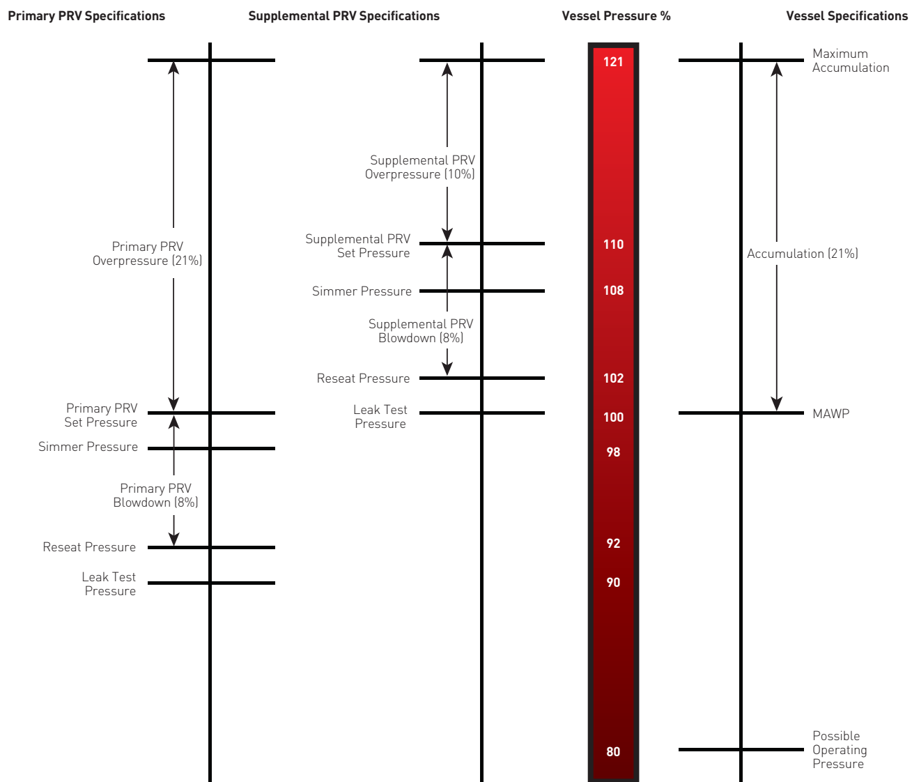
FIGURE 3-11 Typical Section VIII Multiple Valve (Fire Case) Installation
