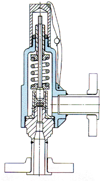
FIGURE 4-18 Inlet Piping Effects on Direct Acting PRV
