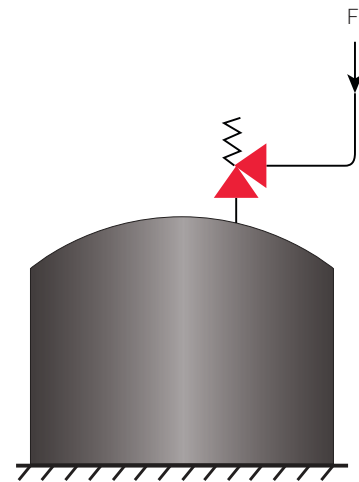
FIGURE 5-7 – OPEN DISCHARGE REACTION FORCE
