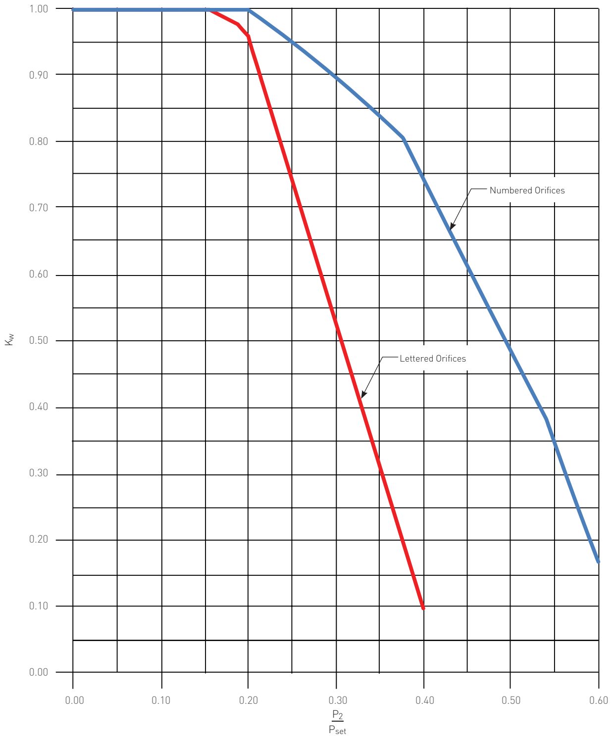
FIGURE 8-19 Anderson Greenwood Series 81P Back Pressure Correction Factor ( K_w ) - Liquid Service
