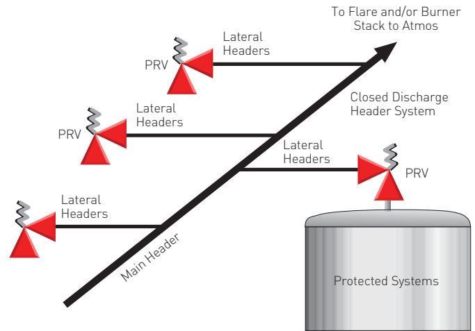
FIGURE 3-14 PRV Discharge Piping Example
