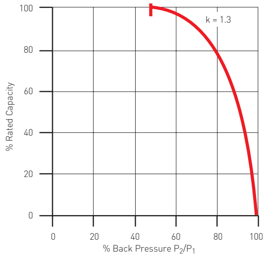
FIGURE 4-38 Sonic to Subsonic Flow Transition
