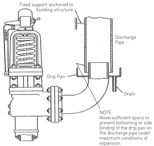
FIGURE 3-6 Recommended ASME Section I Piping Arrangement
