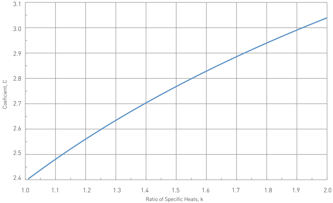
FIGURE 8-30 Gas Constant
