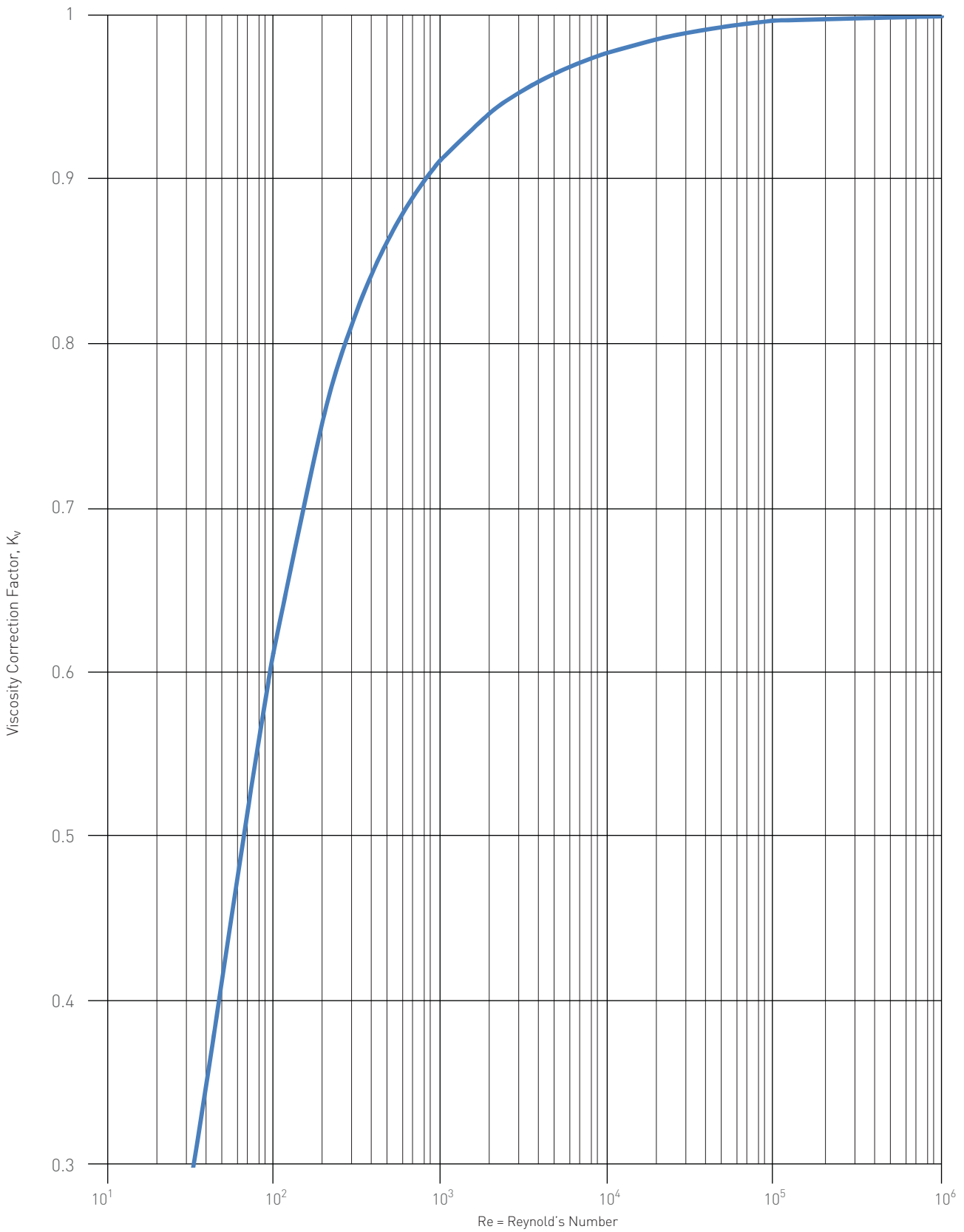
FIGURE 7-29 Viscosity Correction Factor ( K_v )
