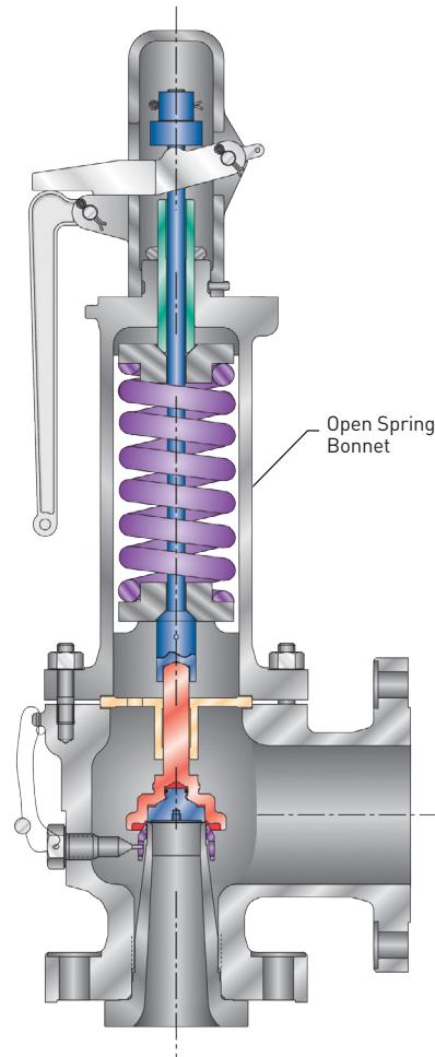
FIGURE 4-15 Open Bonnet Direct Spring PRV
