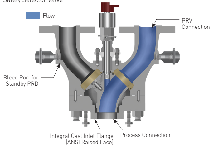
FIGURE 3-5 Safety Selector Valve
