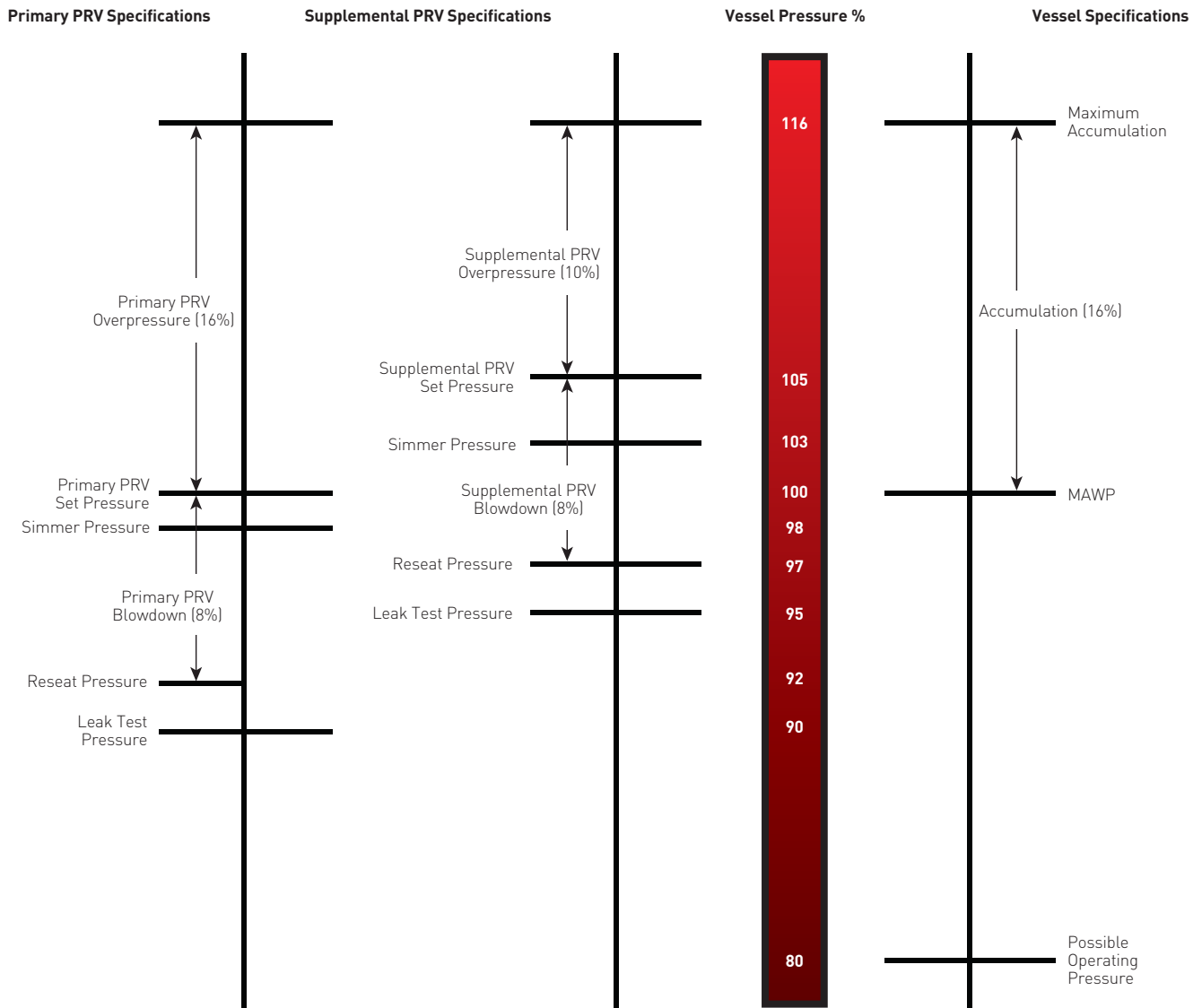
FIGURE 3-10 Typical Section VIII Multiple Valve (Non-Fire Case) Installation
