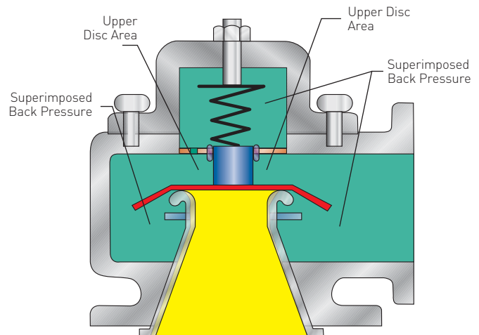
FIGURE 4-22 Superimposed Back Pressure in a Conventional Direct Spring Loaded PRV
