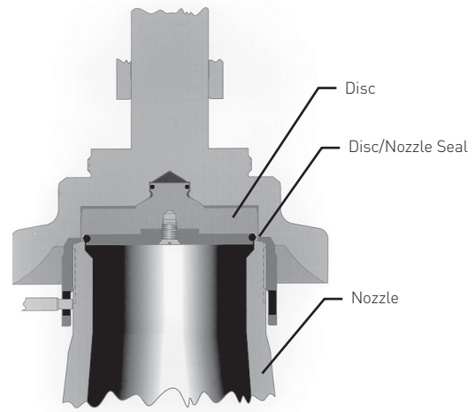
FIGURE 4-13 Metal Seated Direct Spring PRV
