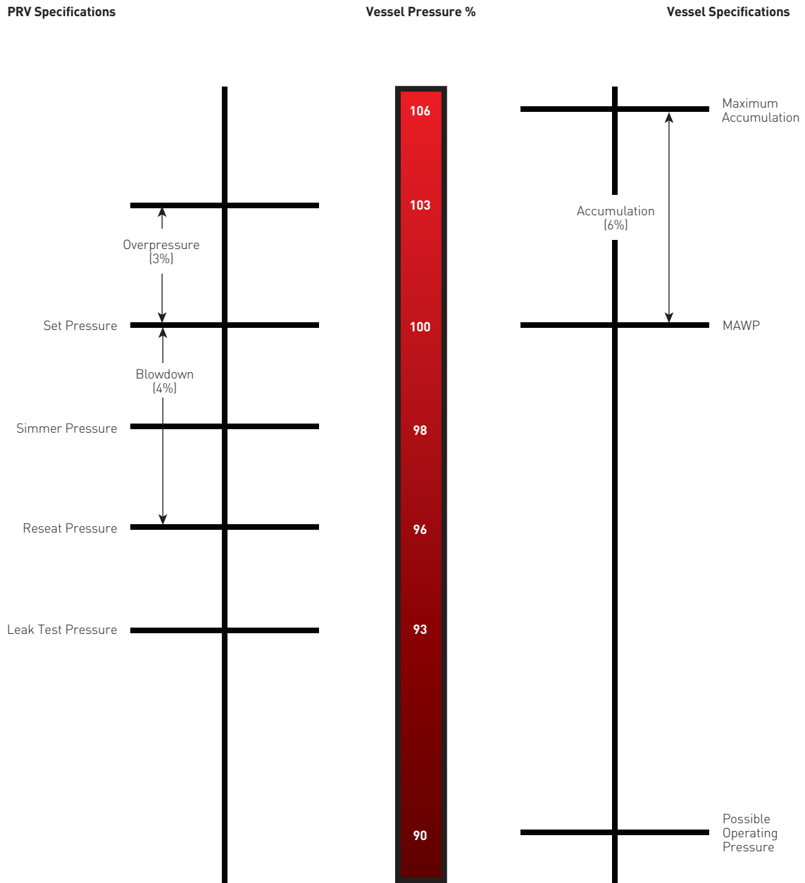
FIGURE 3-1 Typical Section I Single PRV Installation
