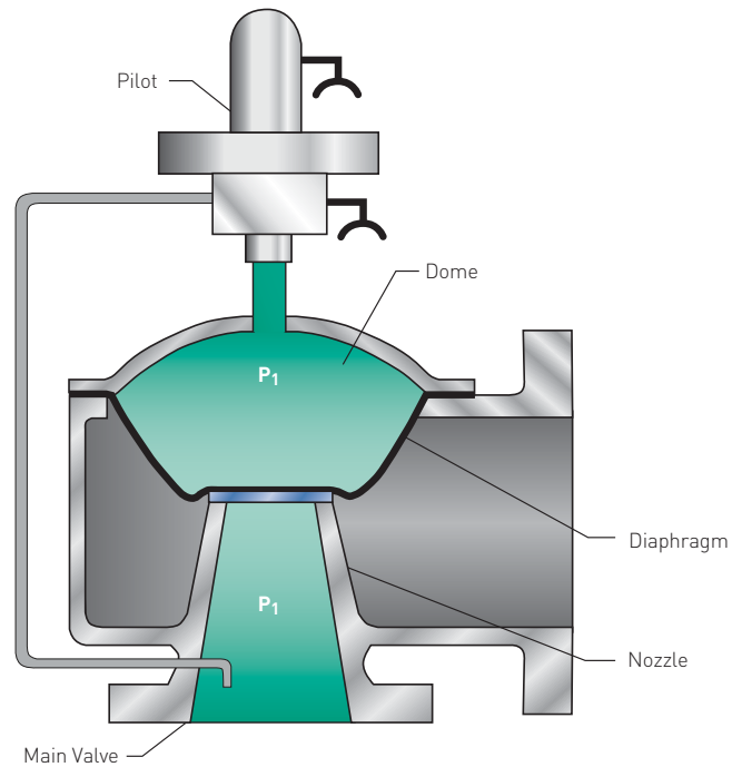
FIGURE 4-26 Diaphragm Type Pilot Operated PRV
