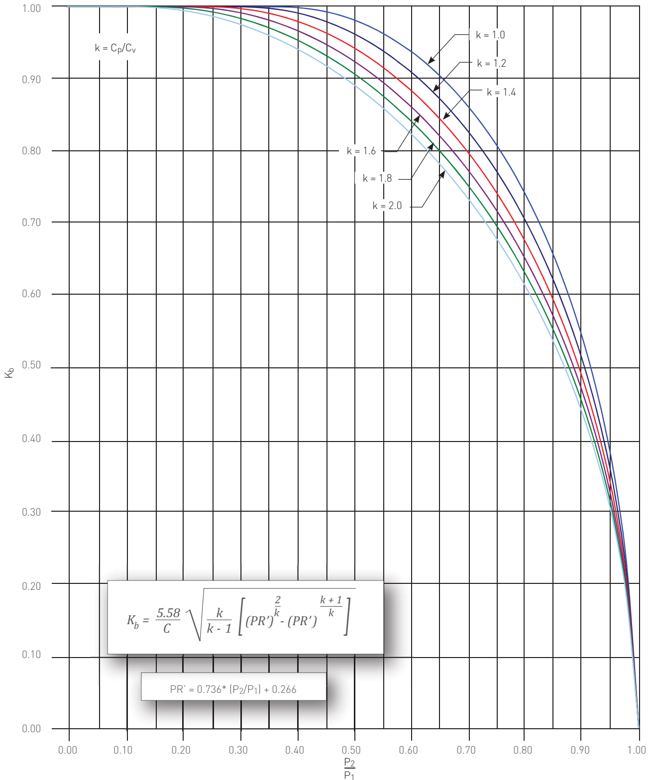
FIGURE 8-13 Crosby Series 900 Conventional Direct Spring PRV Back Pressure Correction Factor ( K_b ) - Gas/Steam Service
