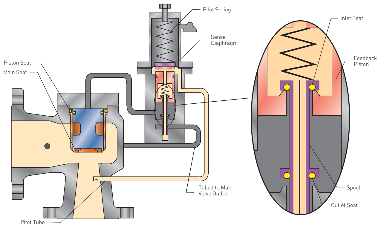
FIGURE 4-33 Modulating Action Pilot Operated PRV (open and in full lift)
