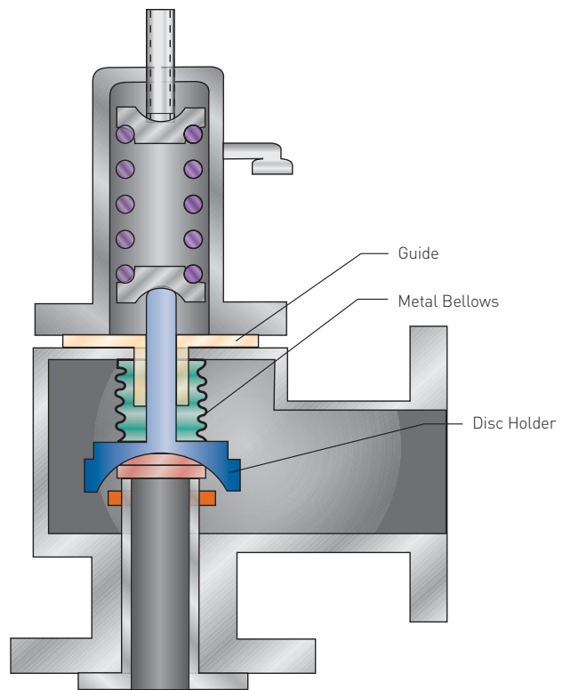
Figure 4-23 Balanced Bellows Direct Spring PRV
