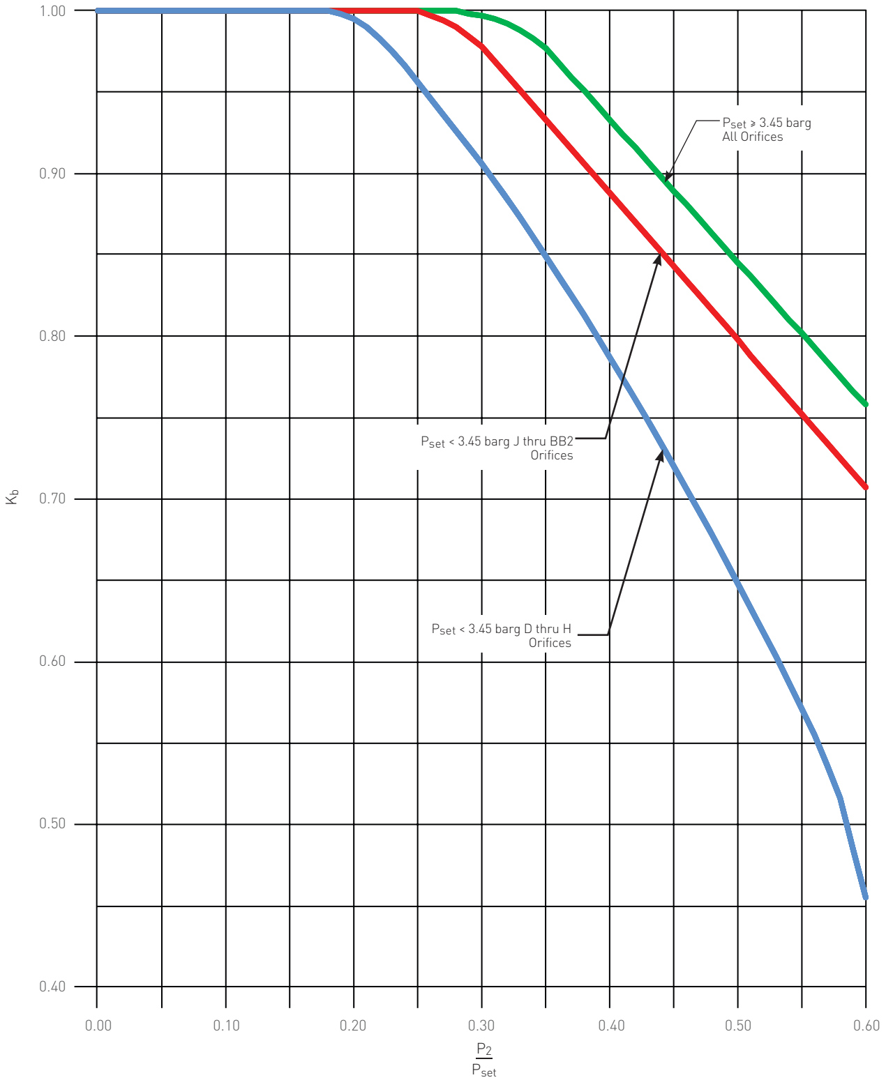
FIGURE 8-10 Crosby Series JBS-E/JLT-JBS-E/JB-TD Balanced Bellows Direct Spring PRV Back Pressure Correction Factor ( K_b ) - Gas/Steam Service
