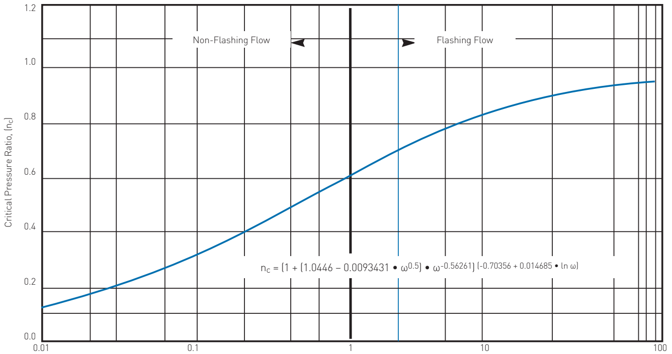
FIGURE 5-3 Omega Parameter, \omega Critical Pressure Ratio for Two-Phase Flow
