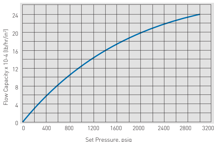
FIGURE 5-5 ASME Section VIII Appendix 11 Available Mass Flux - Saturated Water
