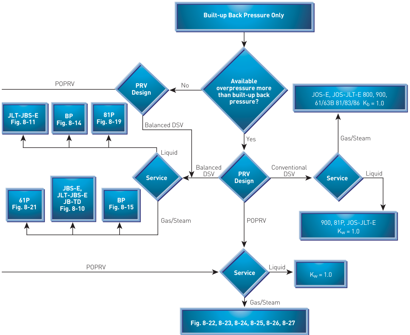
FIGURE 8-4 Valve Selection Recommendations for Built-up Back Pressure Installations
