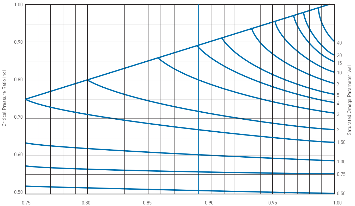
FIGURE 5-4 Saturated Pressure Ratio ( h_s ) Critical Pressure Ratio for Low Subcooled Region Flashing Liquids
