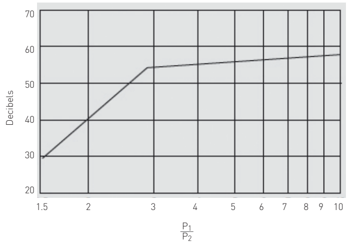
FIGURE 6-5 Sound Pressure Level at 30 meters from Point of Discharge
