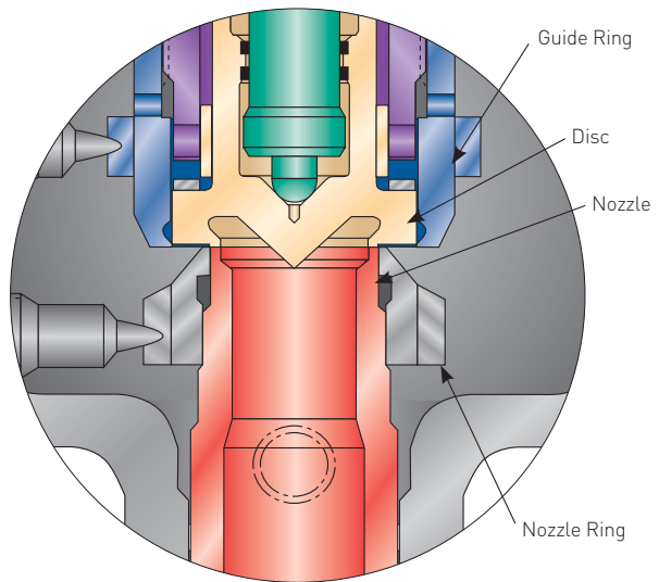
FIGURE 4-9 Effect of Nozzle Ring for ASME Section I Design Safety Valve
