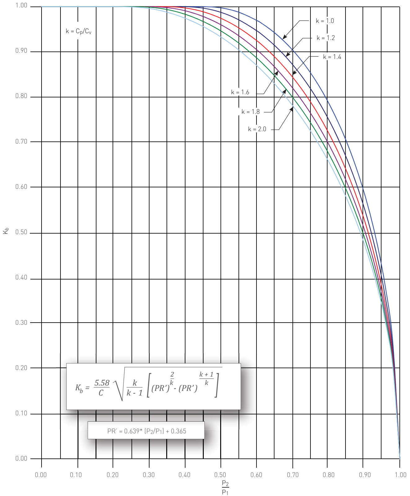
FIGURE 8-12 Crosby Series 800 Conventional Direct Spring PRV Back Pressure Correction Factor ( K_b ) - Gas/Steam Service
