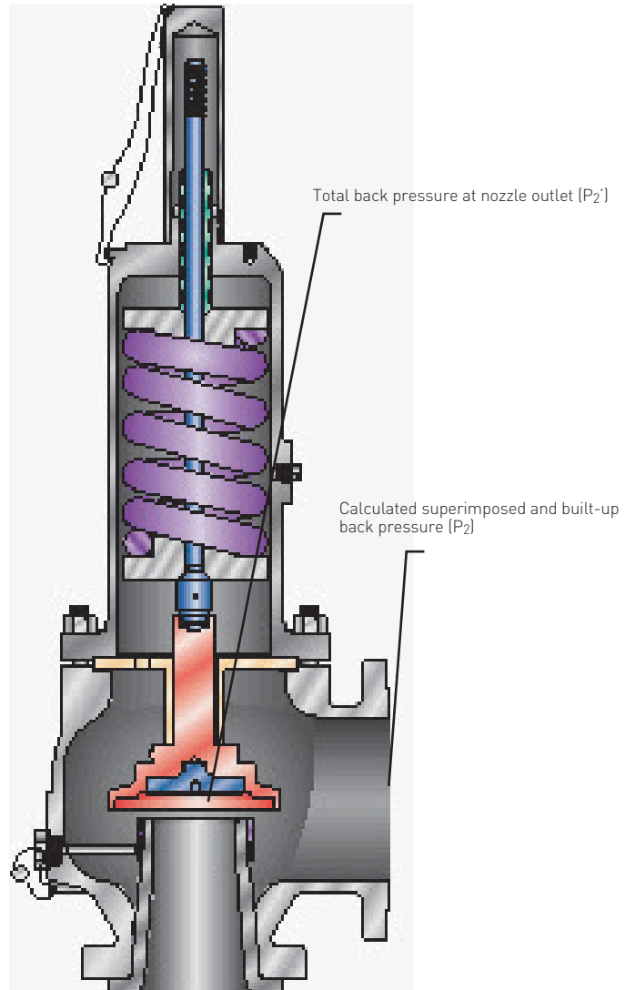
FIGURE 7-3 Relationship of P_2' and P_2
