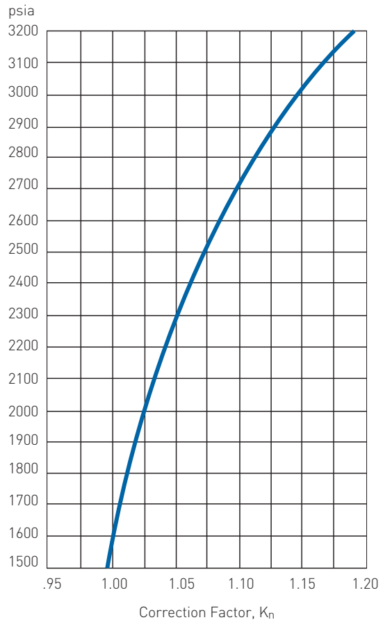
FIGURE 7-28 Correction Factor for High Pressure Steam, K_n
