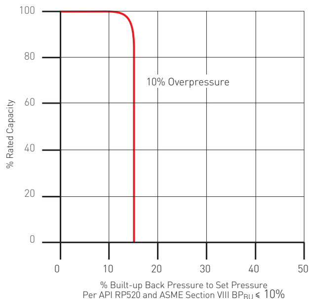
FIGURE 8-2 Effect of Built-up Back Pressure on Conventional PRV
