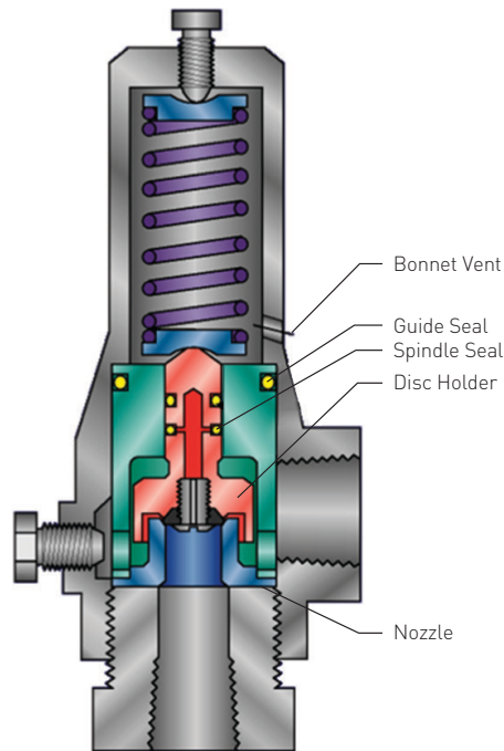
FIGURE 4-24 Balanced Piston Direct Spring PRV
