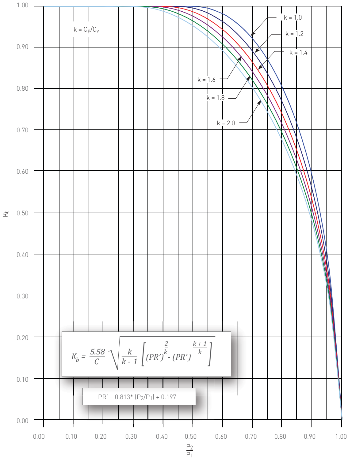
FIGURE 8-23 Anderson Greenwood Series 40 Pilot Operated PRV Back Pressure Correction Factor ( K_b ) - Gas/Steam Service
