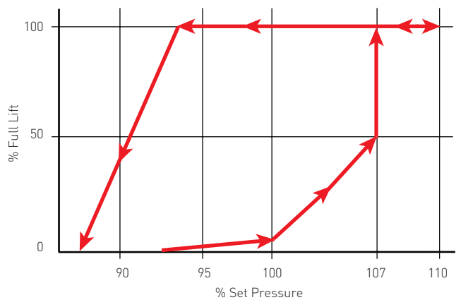
FIGURE 4-12 Typical Relief Valve Lift Characteristic
