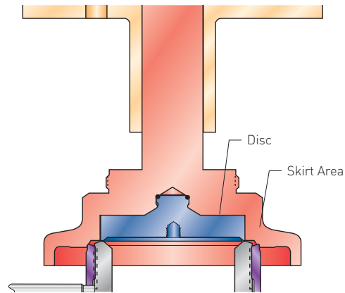
FIGURE 4-6 Section VIII Design Safety Valve Trim
