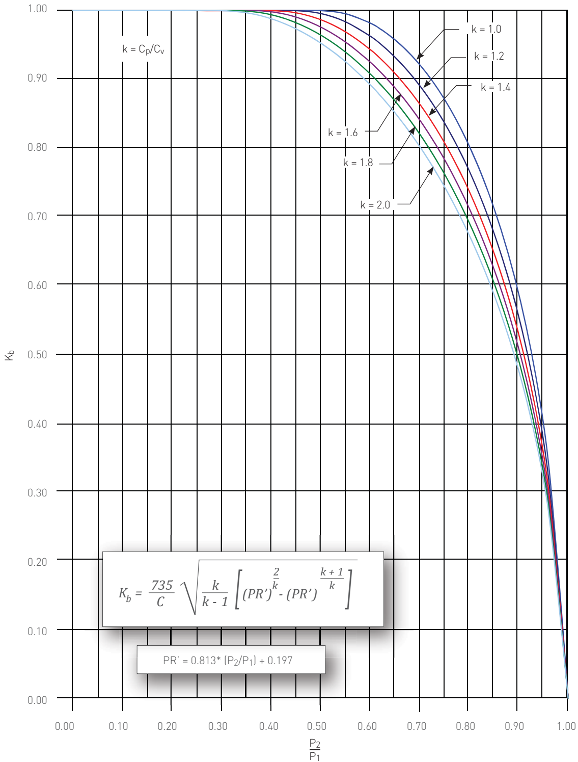
FIGURE 7-23 Anderson Greenwood Series 40 Pilot Operated PRV Back Pressure Correction Factor ( K_b ) - Gas/Steam Service
