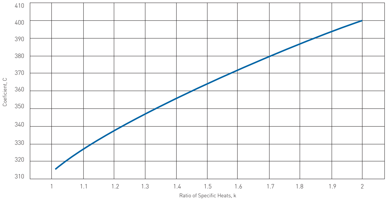
FIGURE 7-30 Gas Constant
