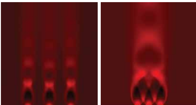
Computational fluid dynamics show jet independence from three properly spaced holes (left). The same three holes spaced too closely (right) show jet interaction, which leads to additional noise. Being able to predict and control jet interaction can reduce the noise produced by up to 40 dBA.
