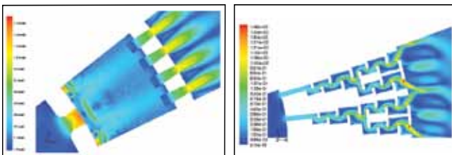
A top-down look at flow through Fisher WhisperFlo trim (left) using computational fluid dynamics illustrates the independence of fluid jets as they exit the cage. In contrast, the exit jets of some tortuous path trims (right) impinge upon one another in pairs, creating an additional noise source.
