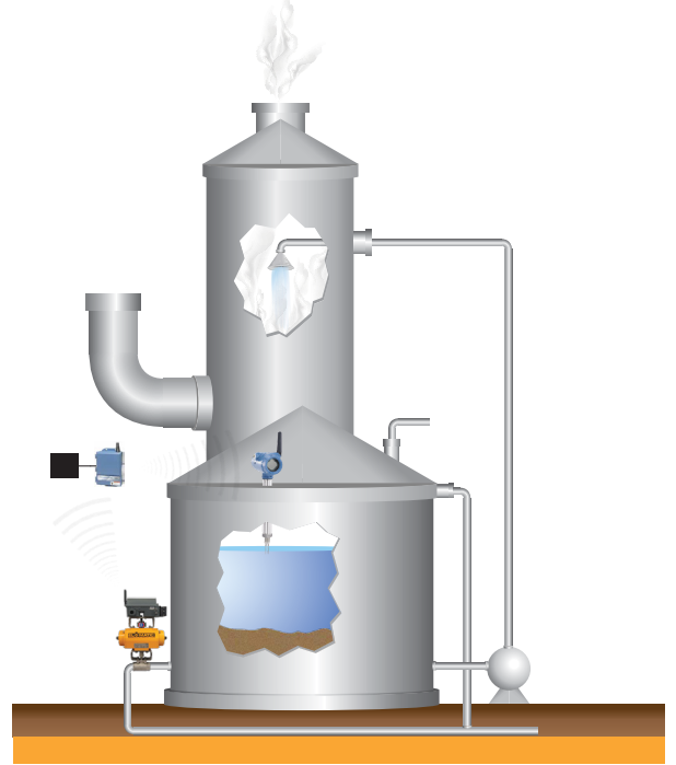
The Fisher 4320 Wireless Position Monitor with On/Off Control Output and Rosemount 2160 Wireless Vibrating Fork Liquid Level Switch were integrated into the DeltaV control logic to provide traditional automation efficiency, but without the traditional cost of engineering and installation of wired instruments and final control elements.
