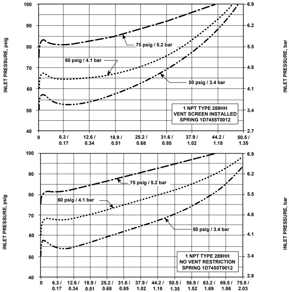
CAPACITIES IN THOUSANDS OF SCFH / Nm 3 /h OF 1.56 SPECIFIC GRAVITY PROPANE GAS AT 14.7 psia AT 60°F / 1.01325 bar AT 0°C
