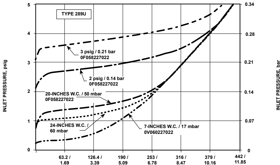
CAPACITIES IN SCFH / Nm 3 /h OF 1.56 SPECIFIC GRAVITY PROPANE AT 14.7 psia AT 60°F / 1.01325 bar AT 0°C
