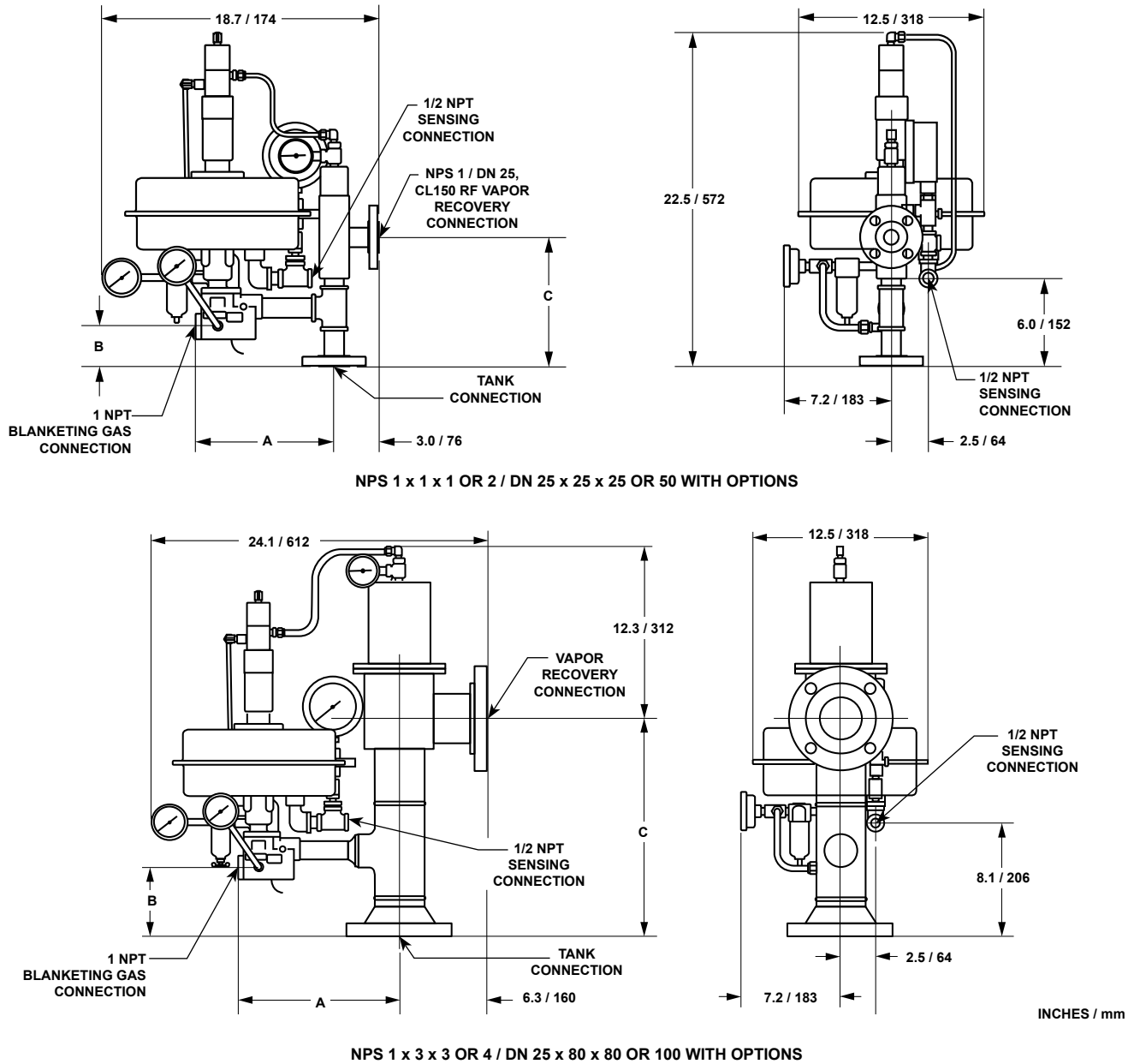
Figure 5. Type ACE97 Pad/Depad Valve Dimensions
