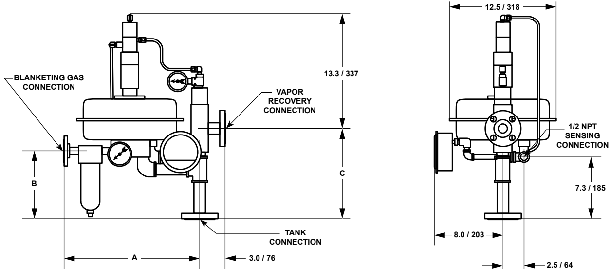
NPS 1/2 x 1 x 1 OR 2 / DN 15 x 25 x 25 OR 50 WITH OPTIONS
