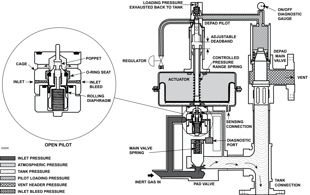
Figure 3. Type ACE97 Pad On / Depad Off
