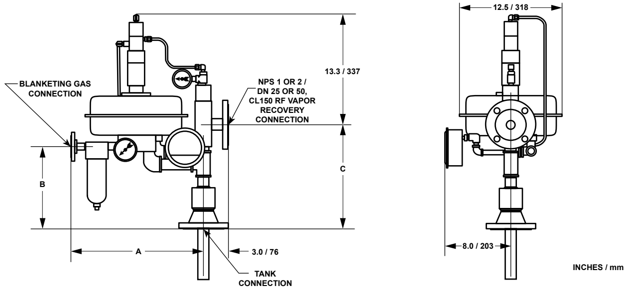
NPS 1/2 x 1 x 2 / DN 15 x 25 x 50 WITH SINGLE ARRAY MANIFOLD
