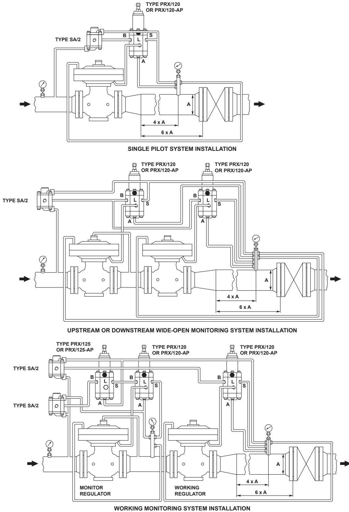
Figure 3. Typical 971 Installation Schematics
