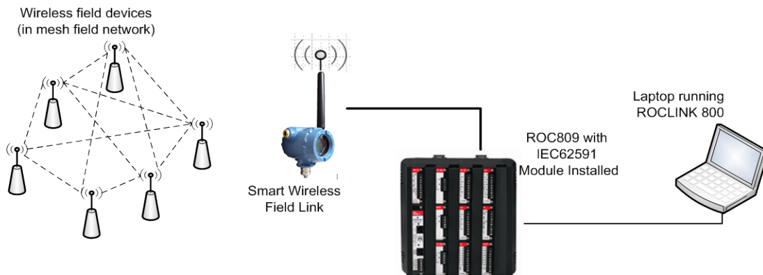
IEC 62591 Interface Self-Organizing Network
