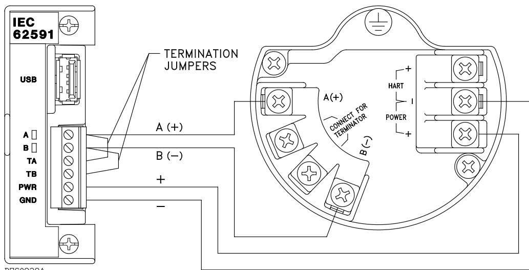
IEC 62591 Interface Wiring Diagram
