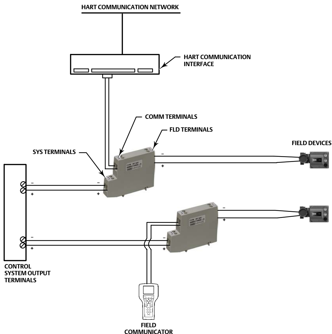
Figure 2. Typical Fisher HF340 HART Filter Installation
