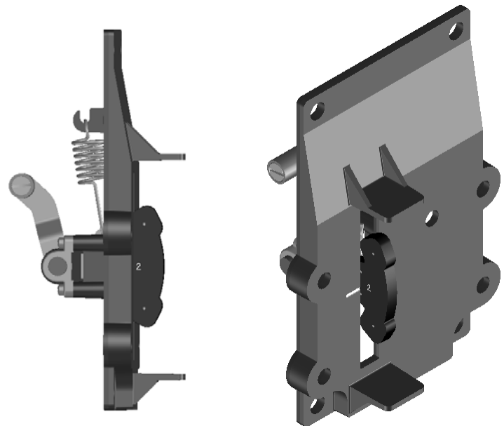
Figure 1. Arced Feedback Assembly For 1051/1052 size 20-33
