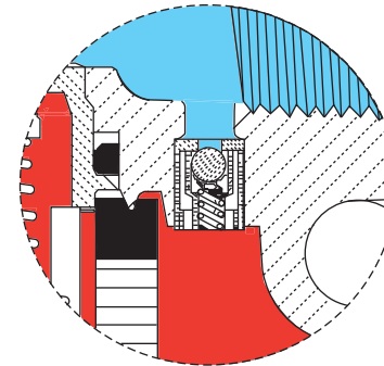
SMART BLEED OPTION FOR TYPE 67DFR OR 67DFSR
