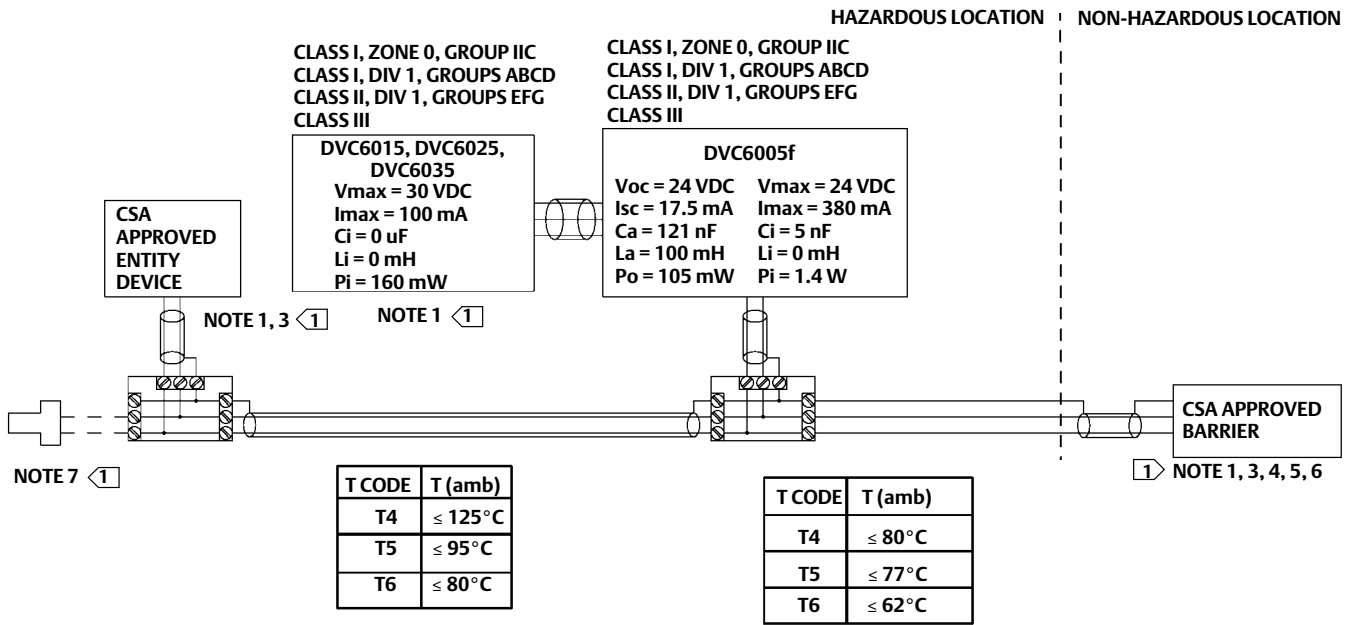
Figure 3. CSA Loop Schematics FIELDVUE DVC6005f and DVC6015, DVC6025, DVC6035
