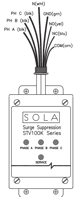
Figure 2: Wiring connections
