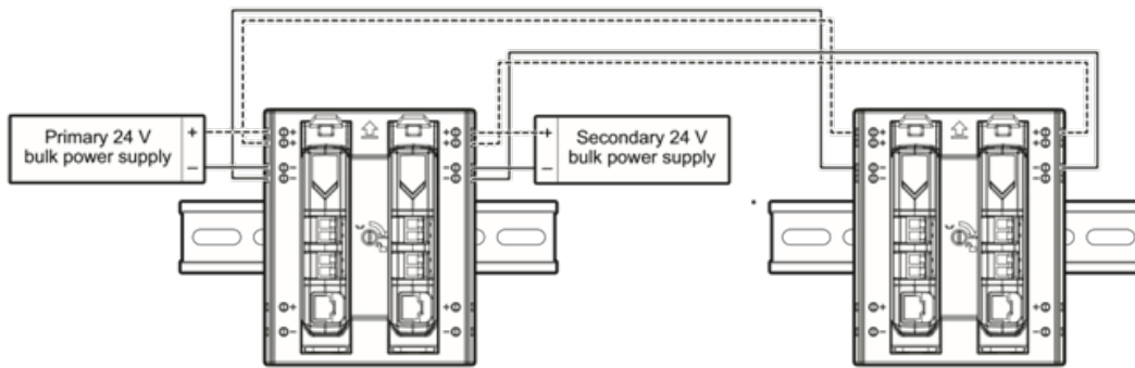
Powering two redundant pairs of Media Converters.
