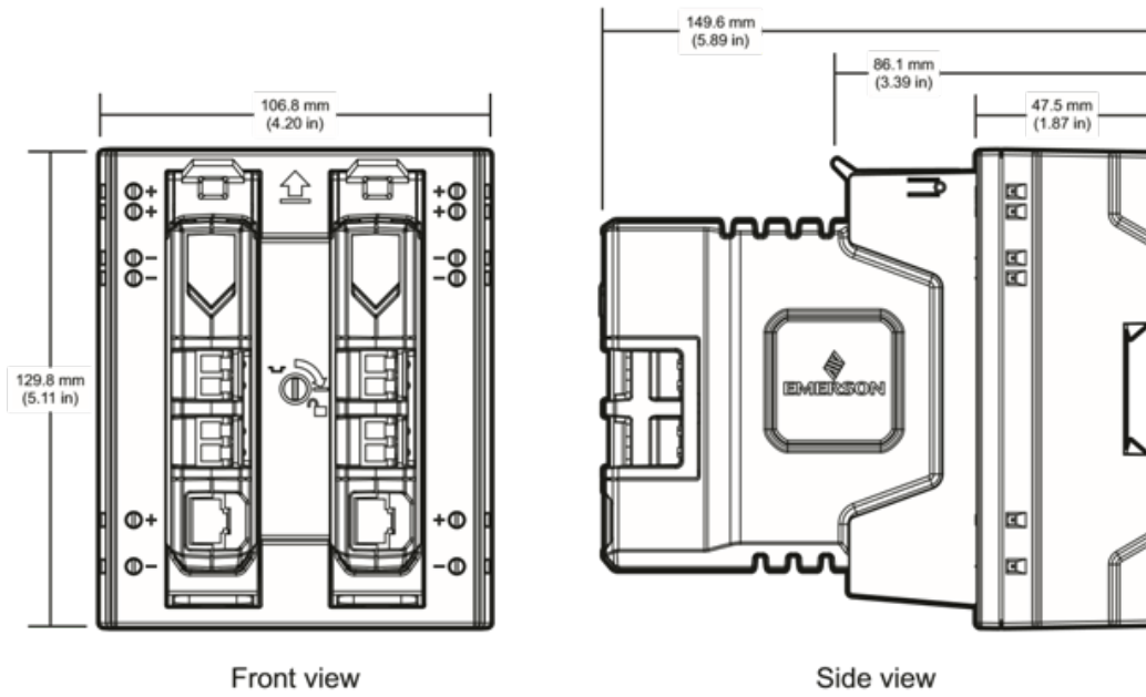
Dimensions of the Media Converters and Carrier.
