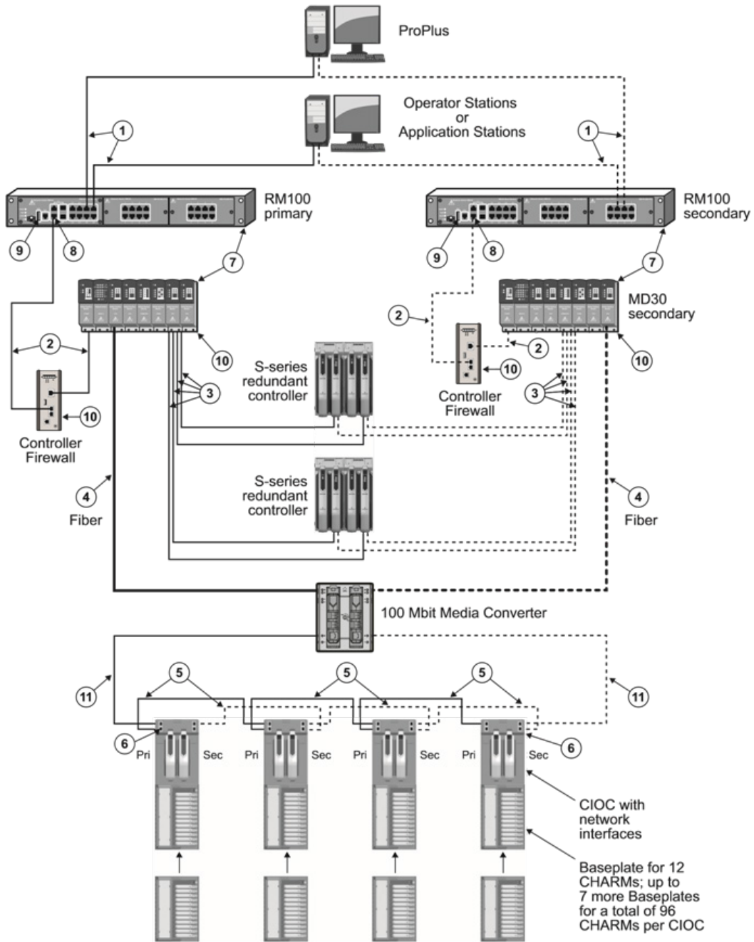
Example 2 - DeltaV Smart Switches with CHARMs I/O, DeltaV Media Converters, and Controller Firewalls.
