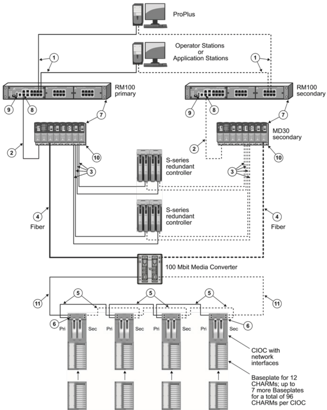
Example 1 - DeltaV Smart Switches with CHARMs I/O and DeltaV Media Converters.
