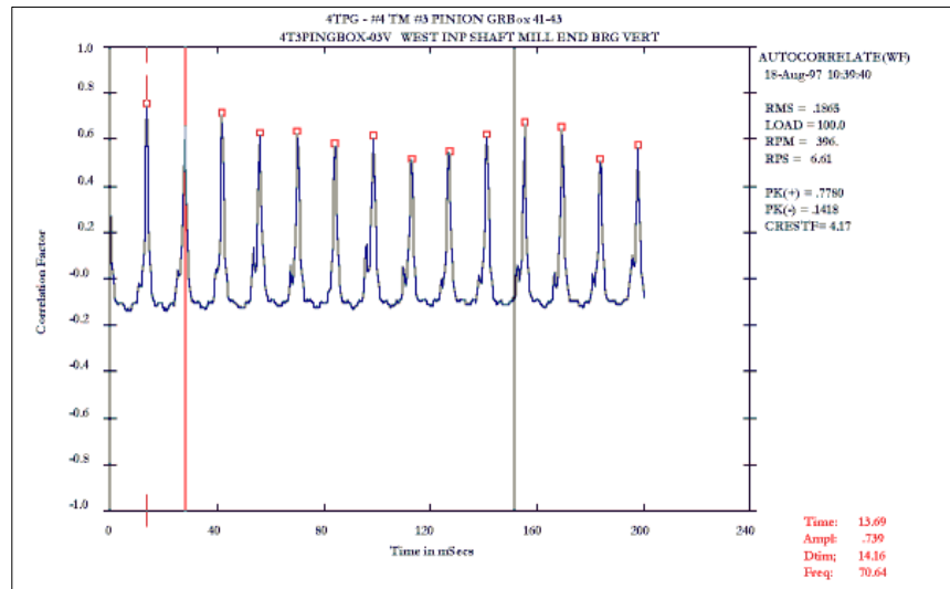
Figure 2: Autocorrelation coefficient from PeakVue time waveform in Fig 1
