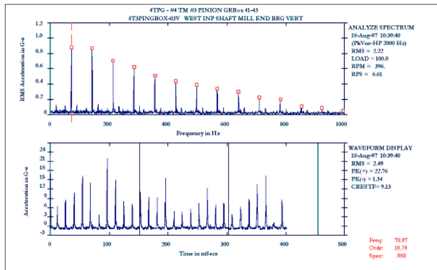
Figure 1: PeakVue Spectra and time waveform from input shaft of pinion stand gearbox
