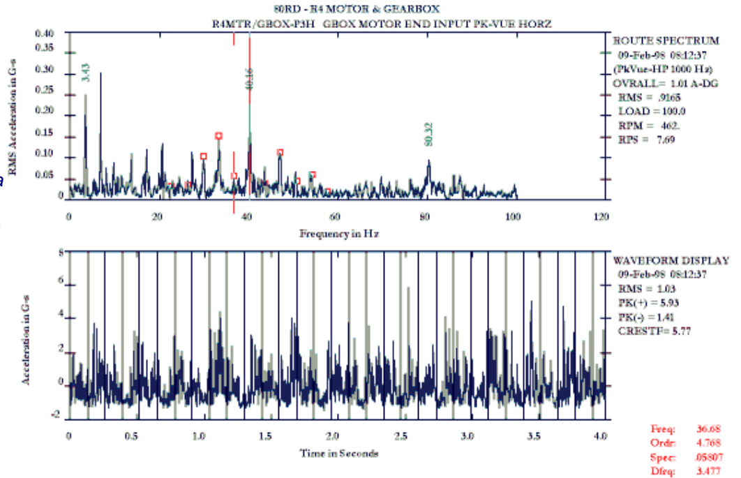
Figure 14. PeakVue Spectra and time waveform from inboard pinion rougher gear box.
