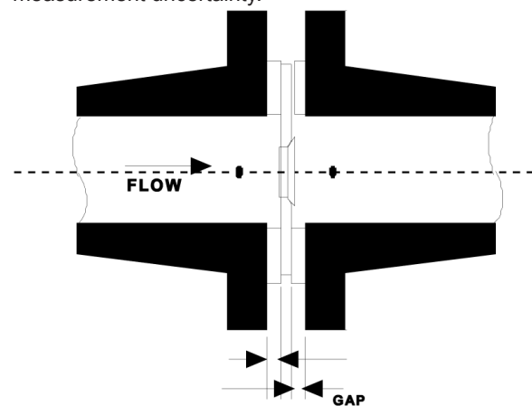
FIGURE 1: RECESSES & PROTRUSIONS
