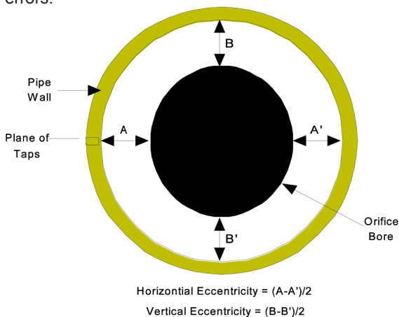
FIGURE 2: ECCENTRICITY MEASUREMENT
