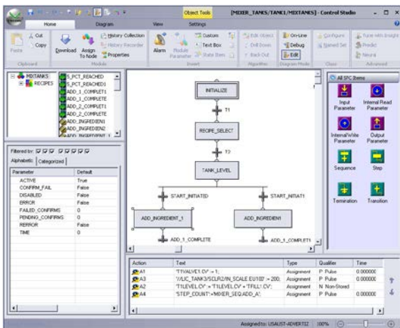
Graphical Sequential Function Chart Configuration
