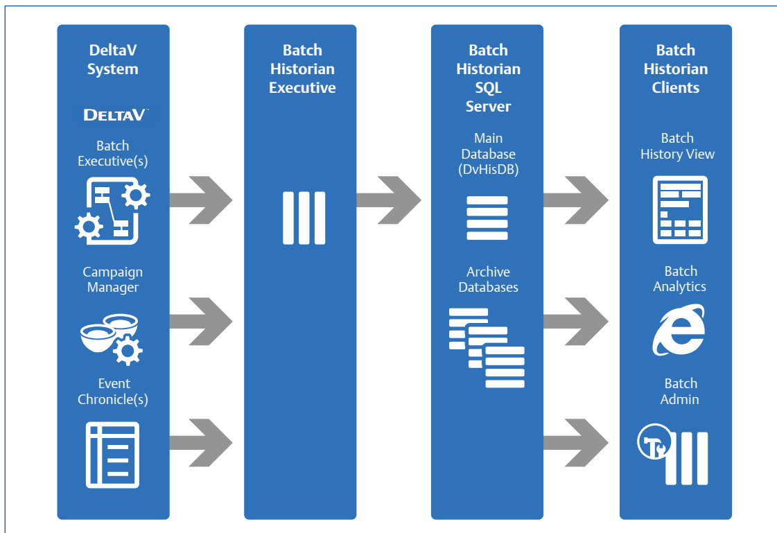
Information flow in the Batch Historian.
