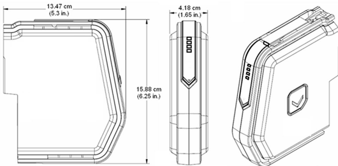
S-series 4-port H1 interface dimensions
