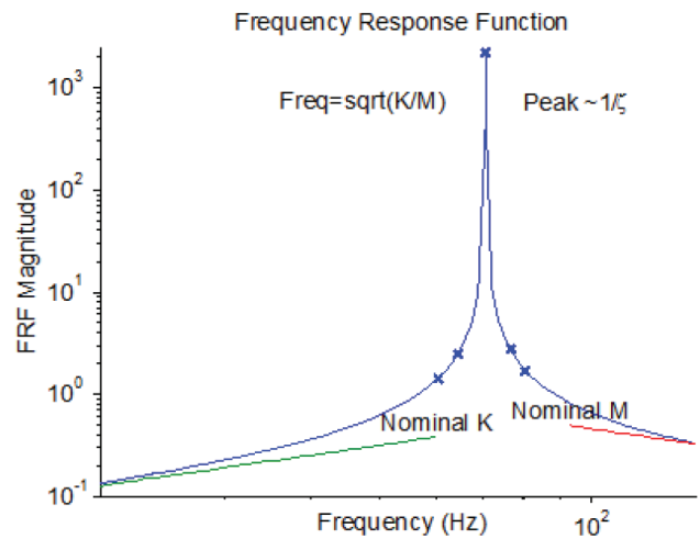
Figure 3. Nominal Frequency Response Function (FRF)
