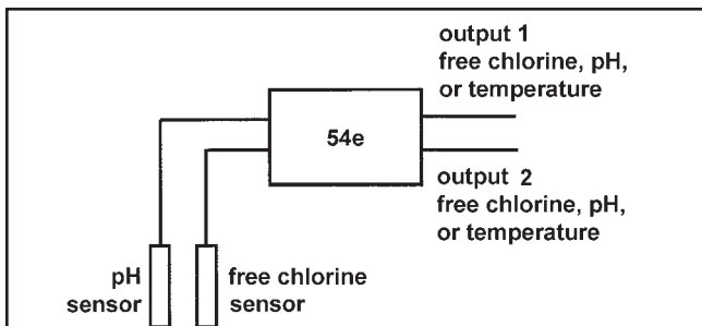
FIGURE 4-1. Configuration of Inputs and Outputs for Free Chlorine
