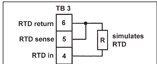
FIGURE 16-5. Simulating RTD Inputs.
