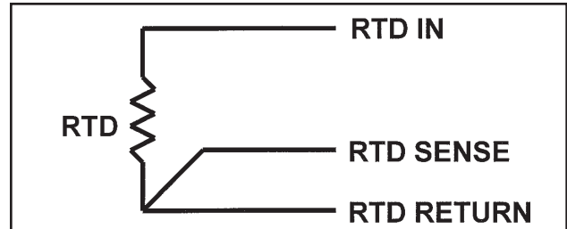
FIGURE 16-4. Three-Wire RTD Configuration.
