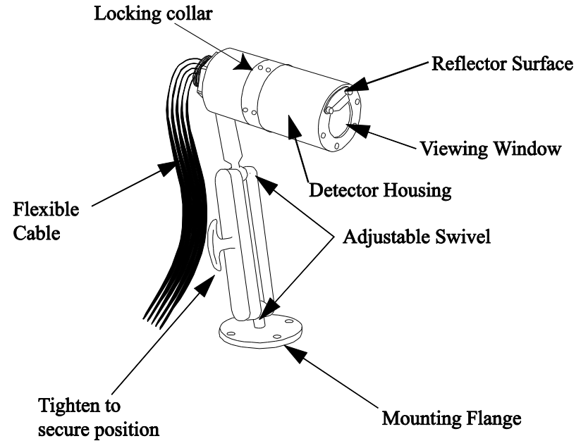
Figure 1: Detector Housing and Swivel Mount
