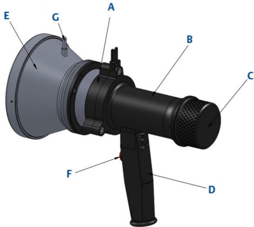
Figure 1-1: Flame simulator side view
