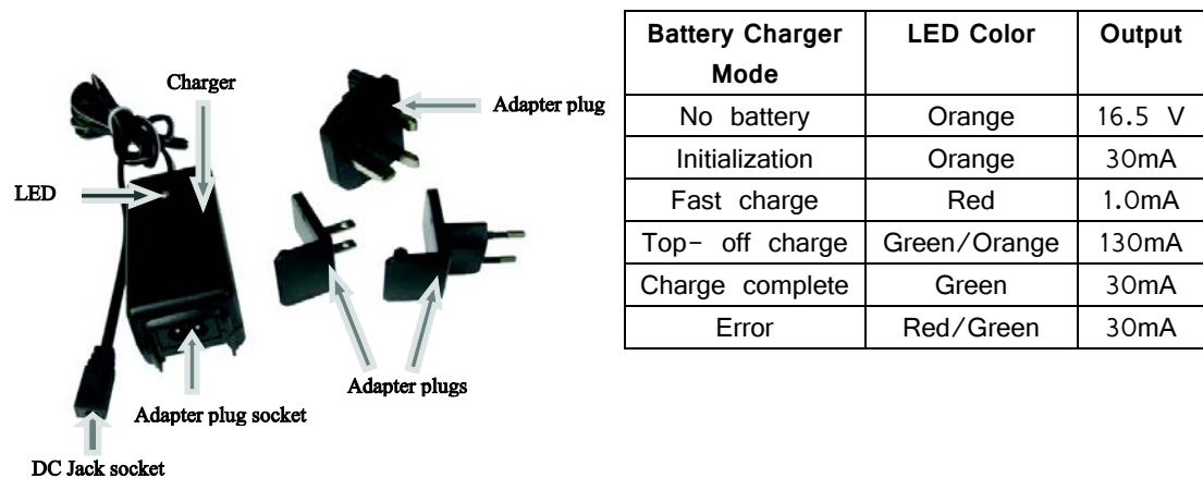
Figure 2-4: Battery Charger
