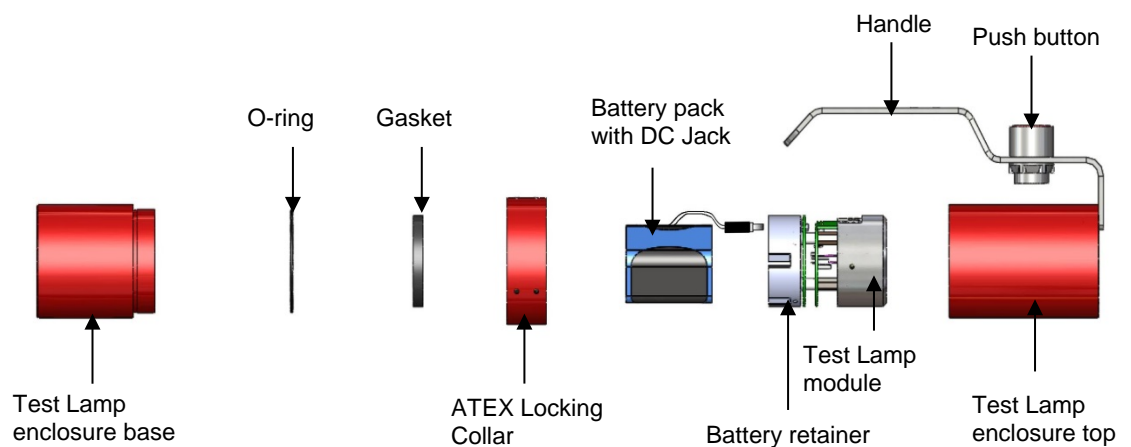
Figure 2-3 Test lamp components
