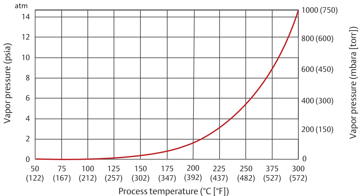
Figure 1-2. Tri-Therm 300 for Vacuum Applications Vapor Pressure Curve
