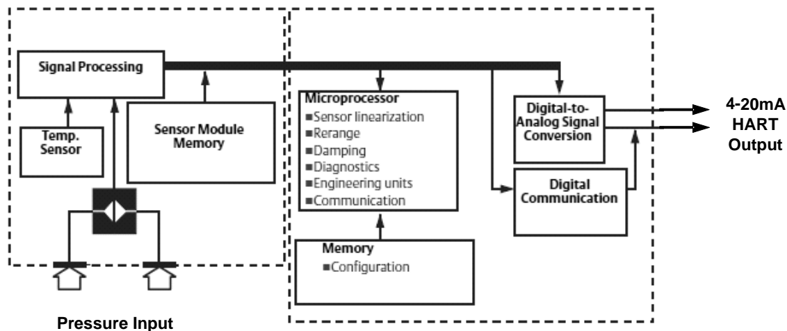
Figure 1 – Rosemount 3051 Pressure Transmitter Block Diagram
