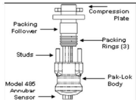
Figure 1: Rosemount 485 Pak-Lok Assembly
