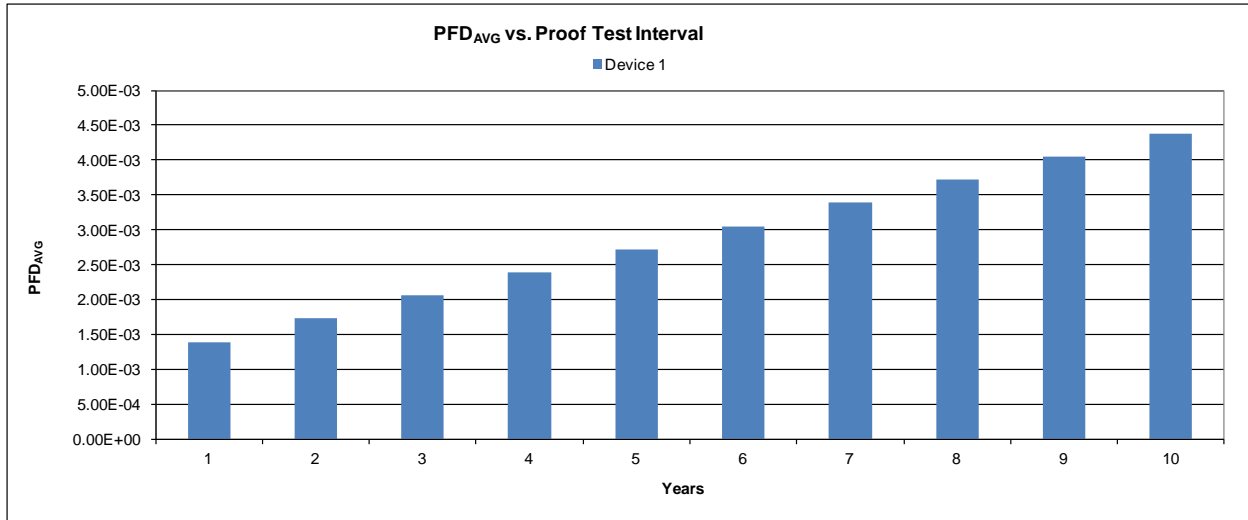
Figure 1: PFD AVG 3144P Temperature Transmitter with single RTD
