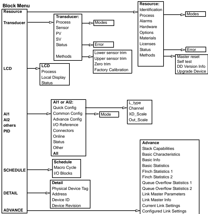
Figure 1. FOUNDATION fieldbus Menu Tree
