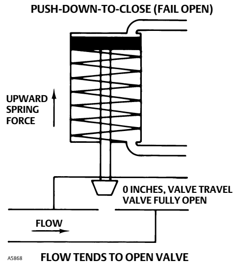
Fisher 585C—Upward Spring Force (Spring Retracts Actuator Rod)
