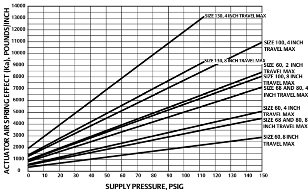
Figure 16. Size 60 through 130 Fisher 585C Actuator Air Spring Effect versus Supply Pressure
