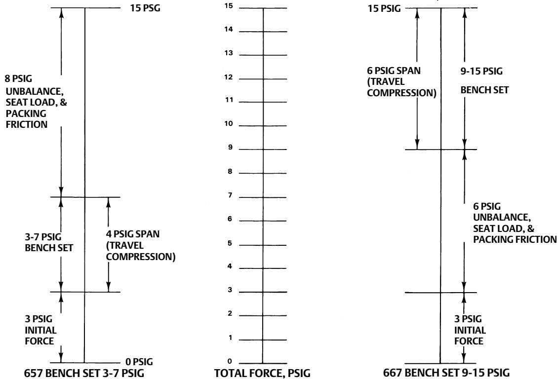
Figure 7. Bench Set
