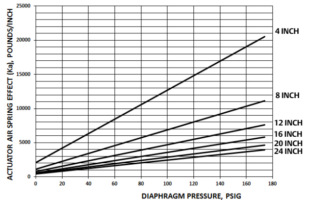
Figure 19. Size 385 Fisher 785C Double Acting Springless Actuator Spring Effect vs Diaphragm Pressure
