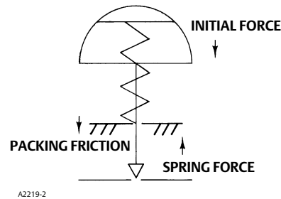
Figure 26. Fisher 657 Actuator Free Body Diagram
