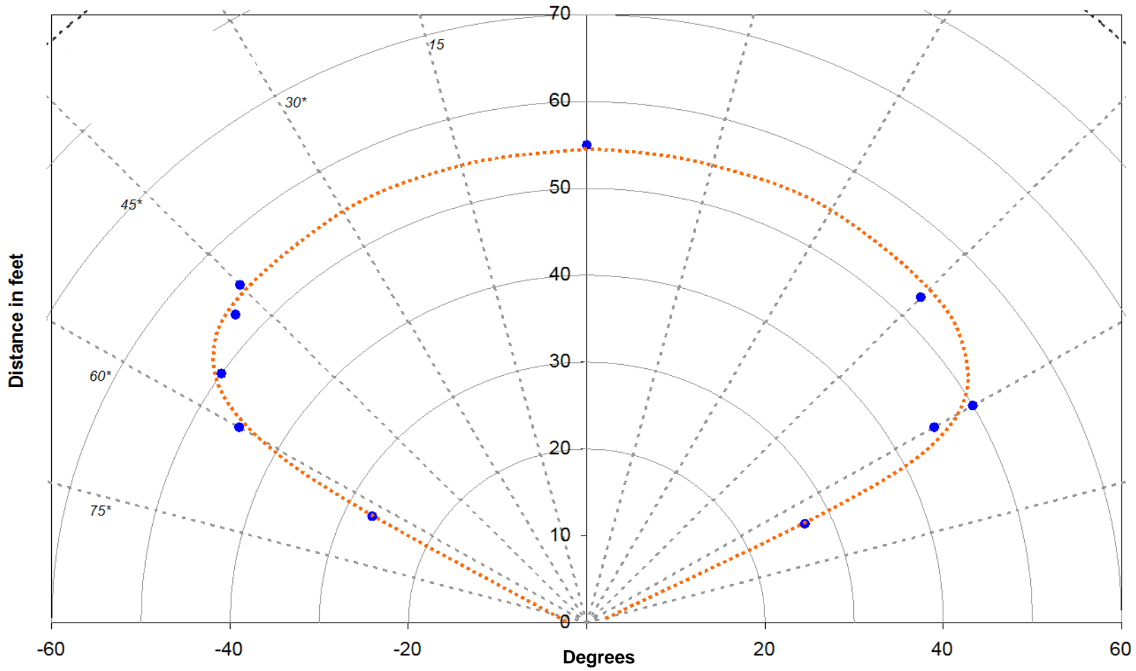
UVIRS-H2 Field of View with a 24" Plume at a distance of 55 feet
