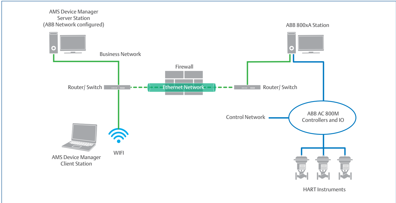
This example architecture shows how AMS Device Manager can be deployed with ABB System 800xA.
