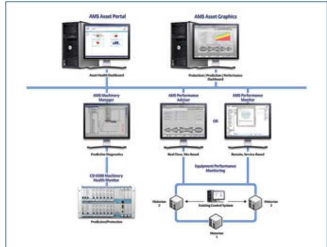
AMS Performance Advisor receives input data from any plant historian via industry-standard OPC protocol.
