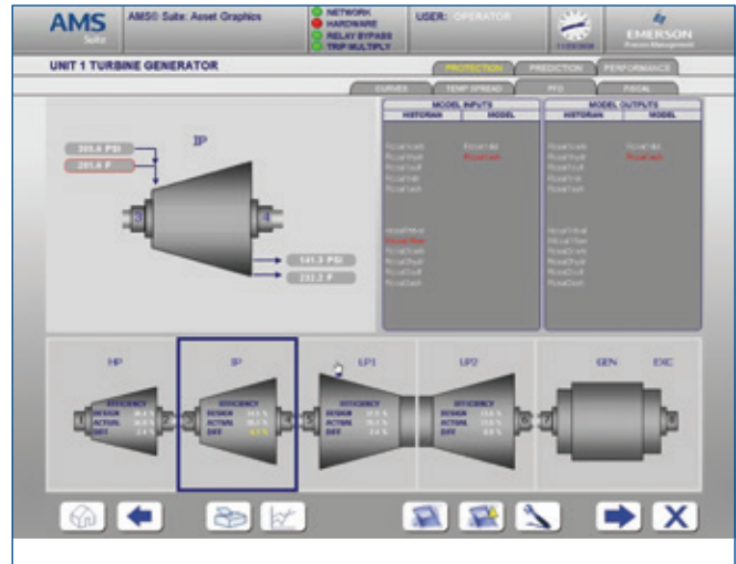
The Process Flow tab provides an easy way to correlate input measurements to the equipment module and determine the impact on model results.
