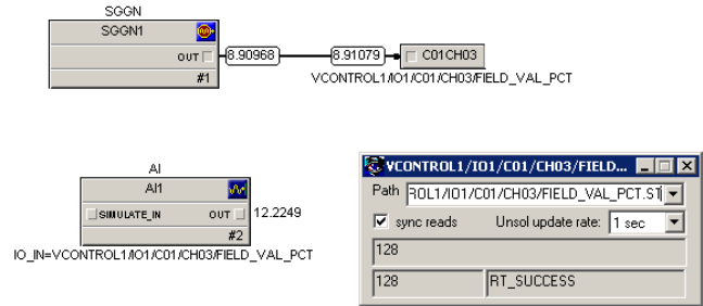
Figure 1 – Referencing Virtual I/O Parameters
