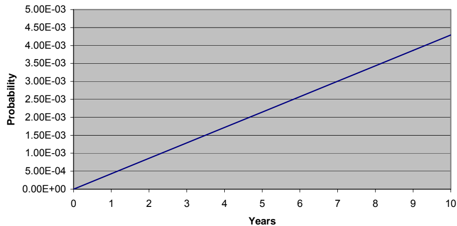
Figure 1: PFD AVG (t) 3051C Pressure Transmitter
