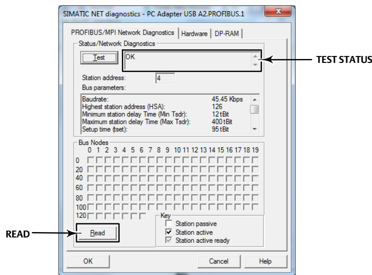
Figure 6. Status/Network Diagnostics
