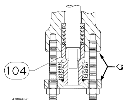
SINGLE PTFE PACKING, OUTBOARD STANDARD DEPTH BOX 8510B
