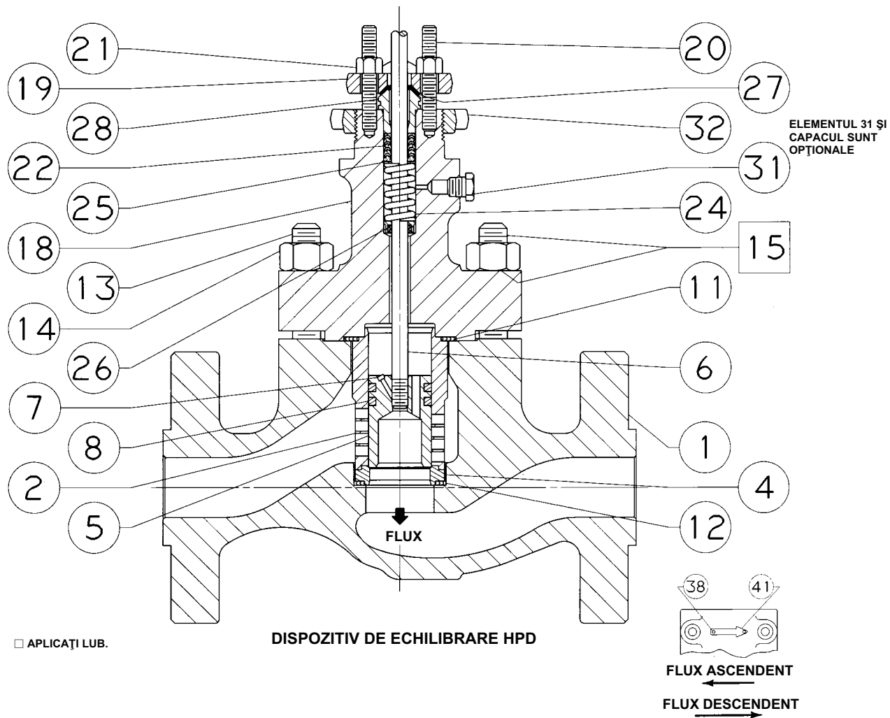
Figura 19. Robinet NPS 2-6 HPD
