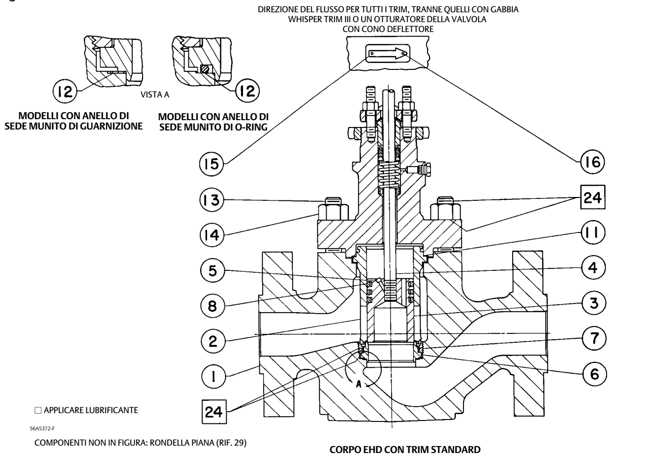
Figura 18. Valvola EHD Fisher
