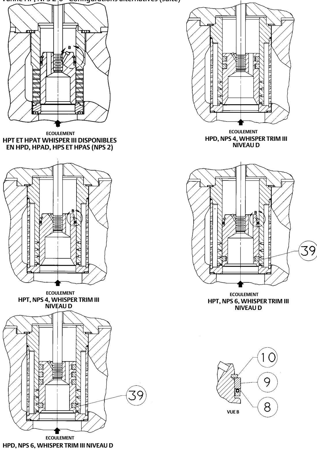
Figure 20. Vanne HP, NPS 2-6 - Configurations alternatives (suite)
