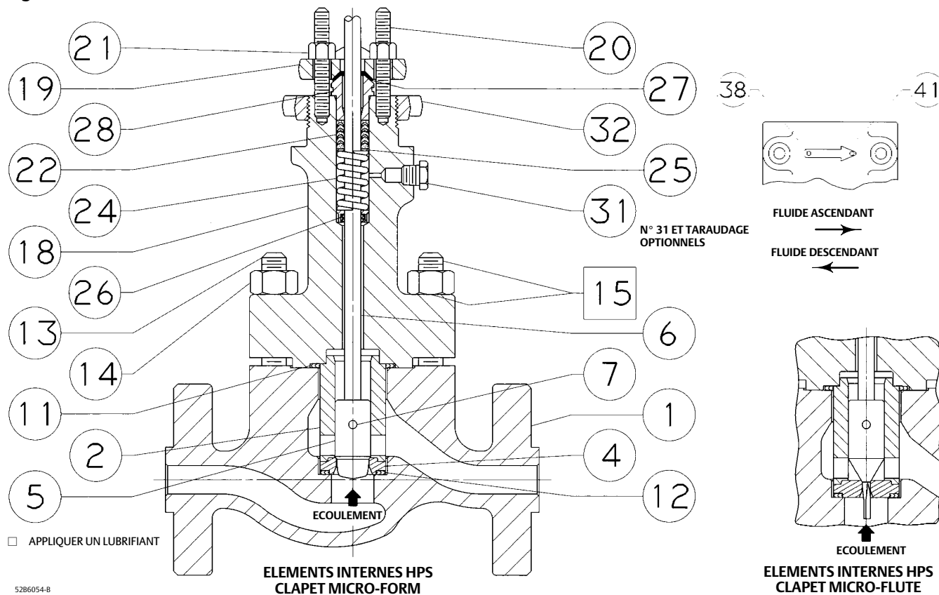
Figure 17. Vanne HPS, NPS 1
