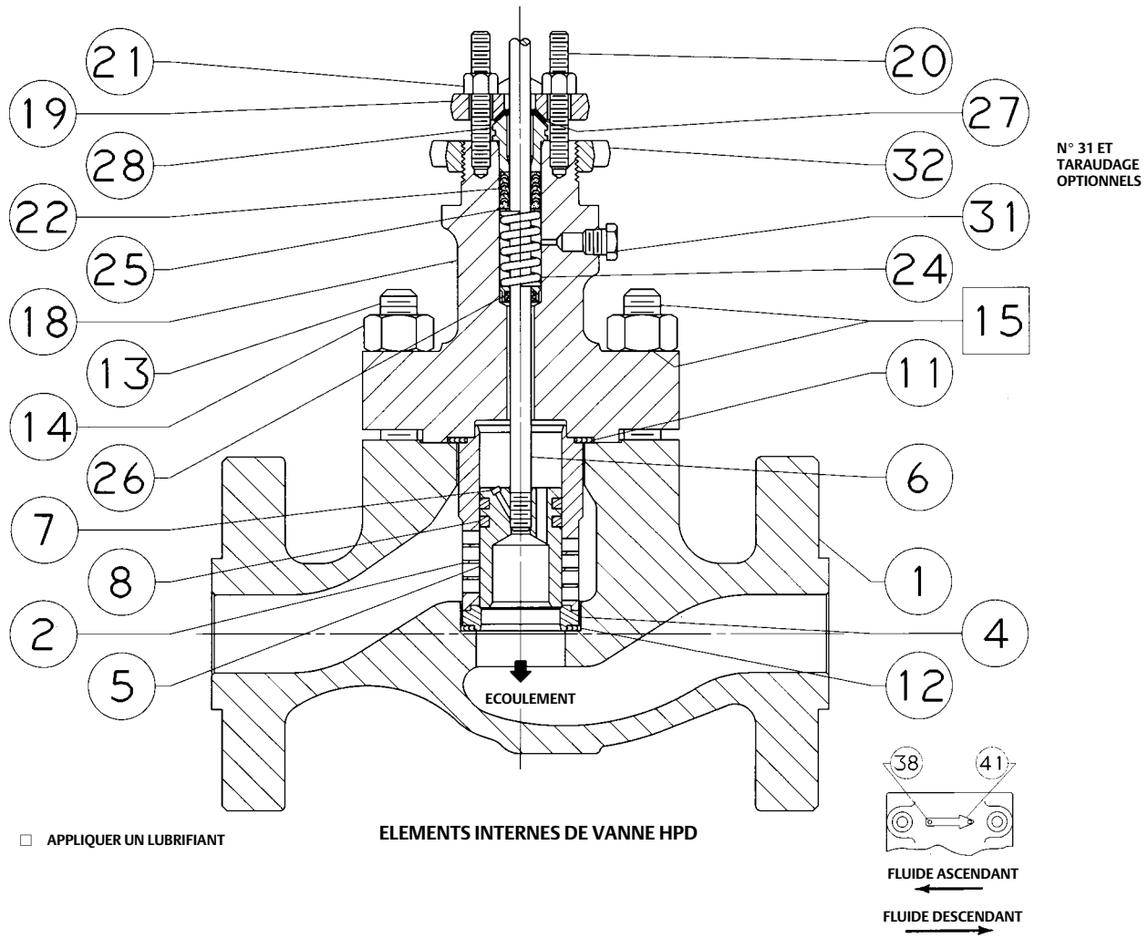
Figure 19. Vanne HPD, NPS 2-6
