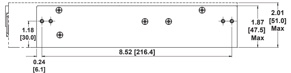
Figure 2: Mechanical Drawing
