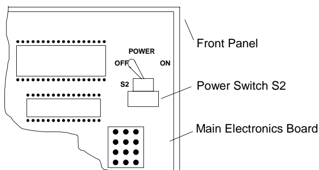
FIGURE 3-1. POWER SWITCH LOCATION
