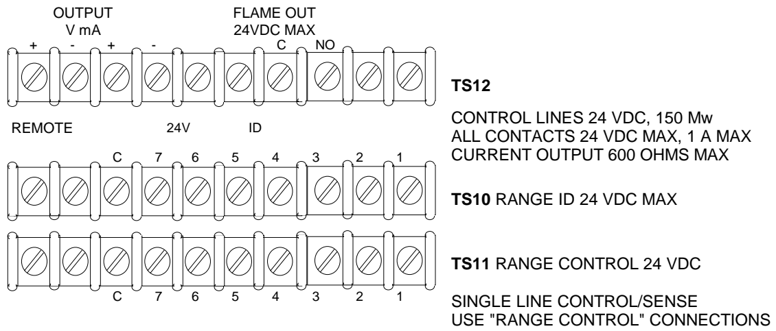
FIGURE 2-2. RANGE CONTROL AND OUTPUT CONNECTIONS
