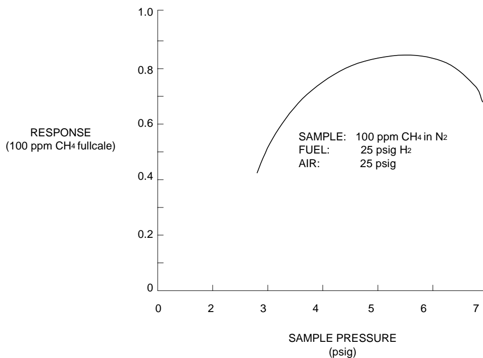
FIGURE 4-1. TYPICAL CURVE OF ANALYZER RESPONSE VS. PRESSURE SETTING ON SAMPLE PRESSURE
