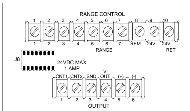
FIGURE 2-1. RANGE INPUT-OUTPUT BOARD
