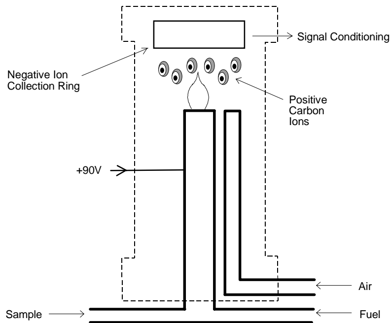
FIGURE 5-1. FLAME IONIZATION DETECTION THEORY
