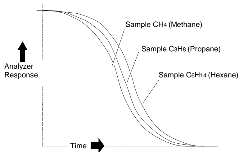
FIGURE 3-2. TYPICAL CURVES OF DOWNSCALE RESPONSE VS. TIME FOR VARIOUS HYDROCARBONS
