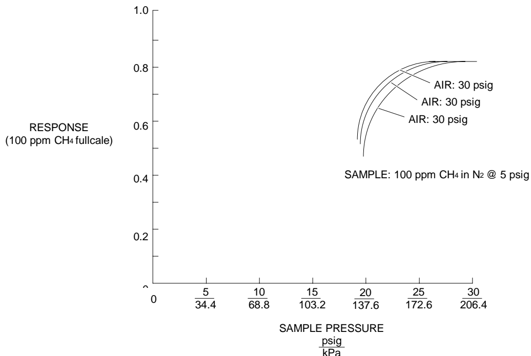
FIGURE 4-2. TYPICAL CURVES OF ANALYZER RESPONSE VS. PRESSURE SETTING ON FUEL PRESSURE REGULATOR
