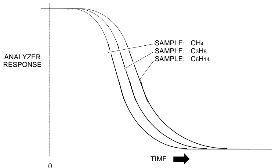
FIGURE 5-2. TYPICAL CURVES OF DOWNSCALE RESPONSE VS. TIME FOR VARIOUS HYDROCARBONS
