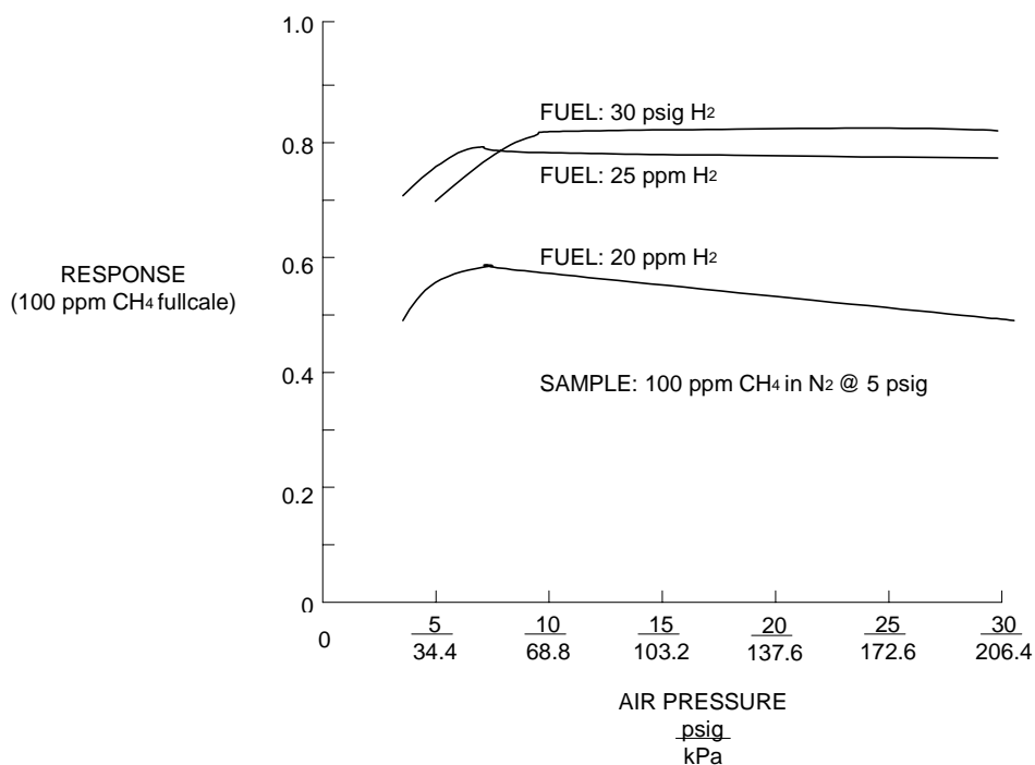
FIGURE 4-3. TYPICAL CURVES OF ANALYZER RESPONSE VS. PRESSURE SETTING ON AIR PRESSURE REGULATOR
