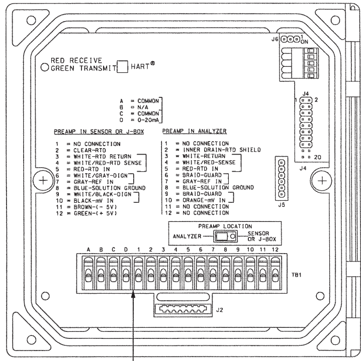
FIGURE 8-2. Junction Box Preampifier Check
