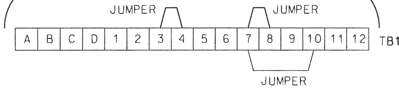
FIGURE 8-3. Controller Preampifier Check
