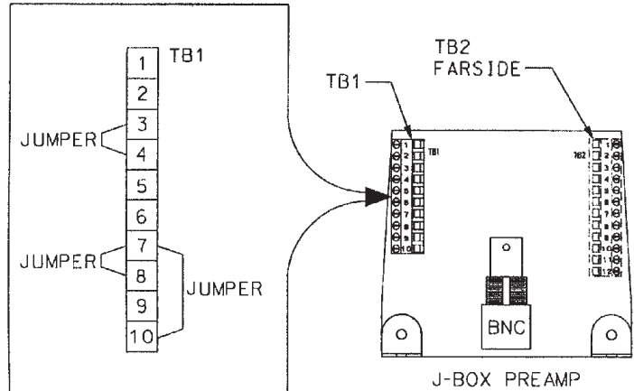
FIGURE 8-2. Junction Box Preampifier Check
