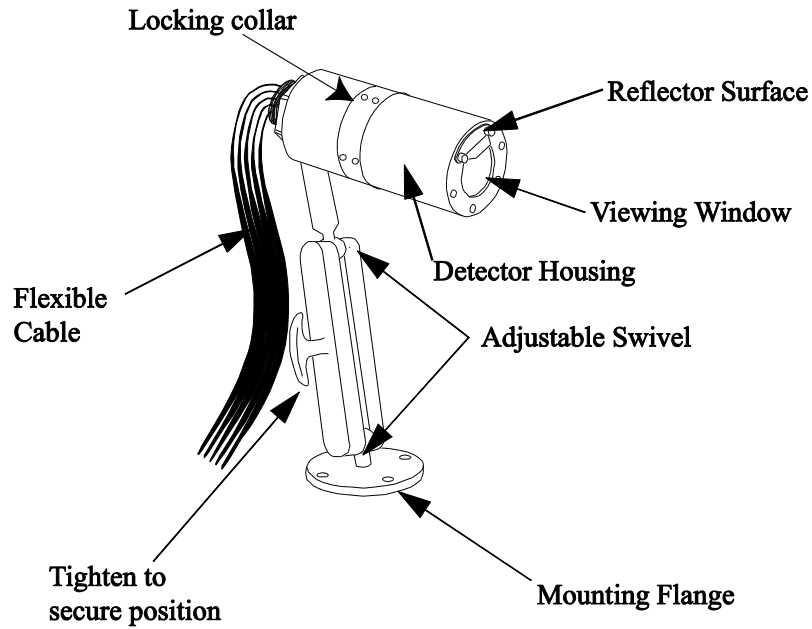
Figure 1: Detector Housing and Swivel Mount
