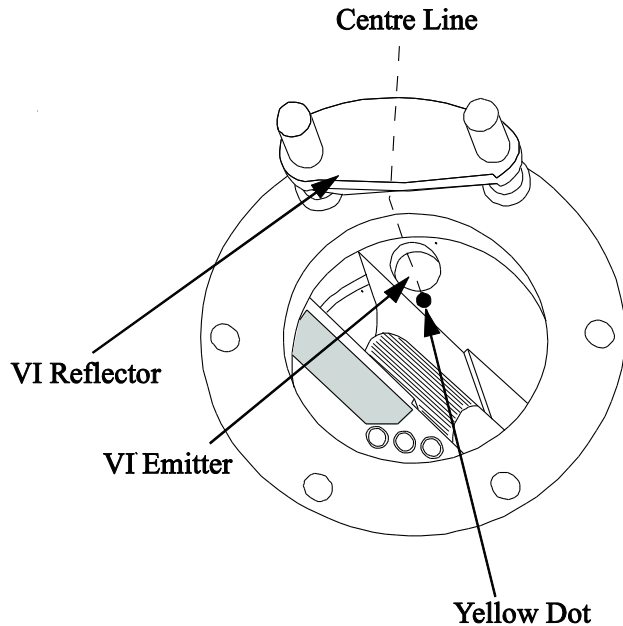
Figure 3: Position of VI Reflector
