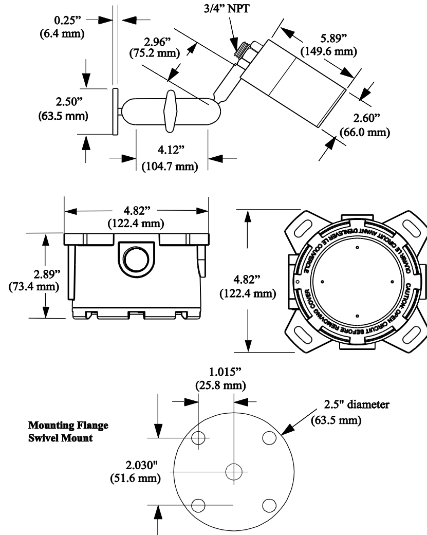
Figure 2: Dimensional Drawing
