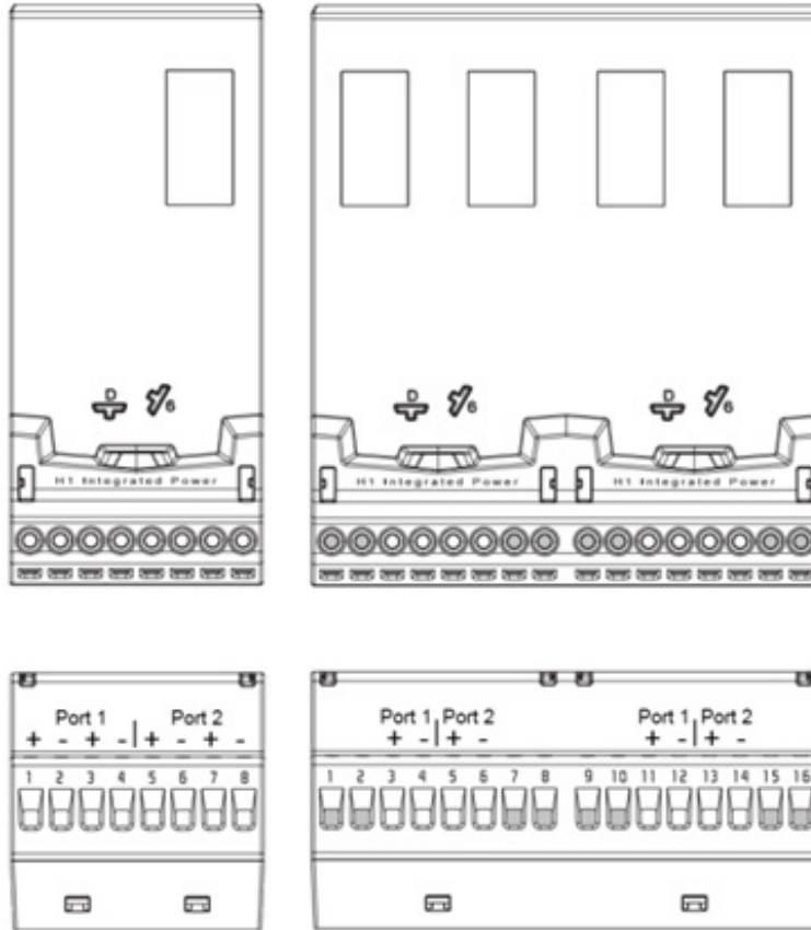
S-series H1 with Integrated power Terminal Blocks
