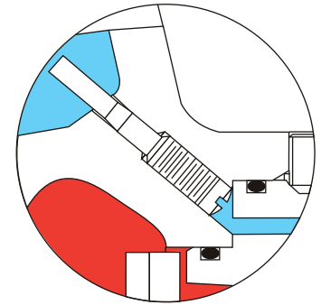
Type VSX-2 with External Registration
