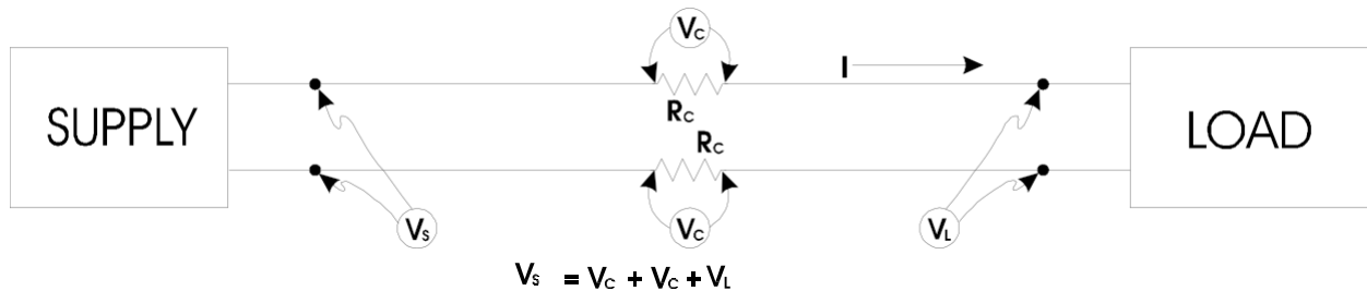
Figure 5-3. Calculating Load Voltage due to Line Resistance
