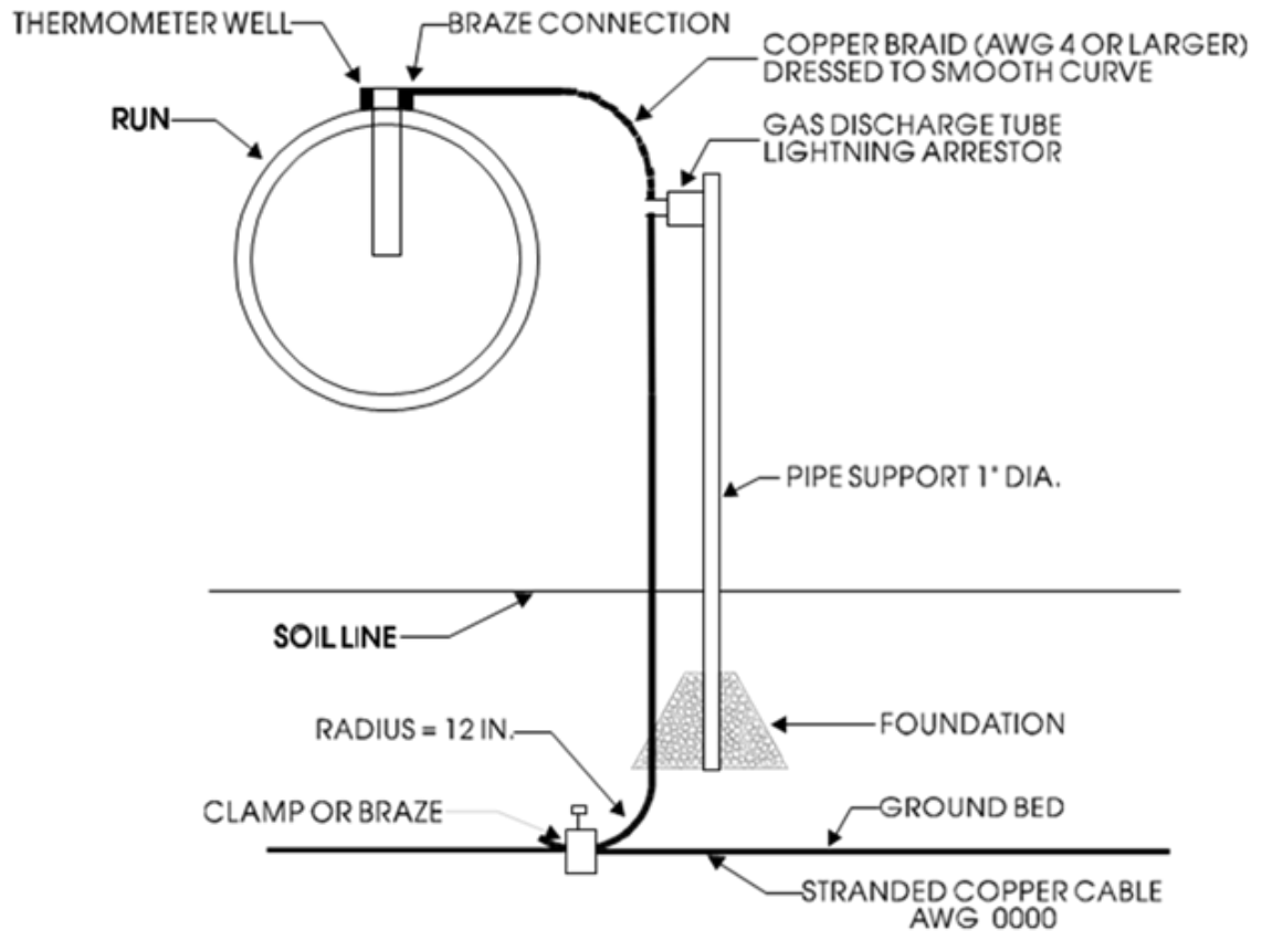
Figure 3-7: Grounding of Thermometer Well in Gas Line
