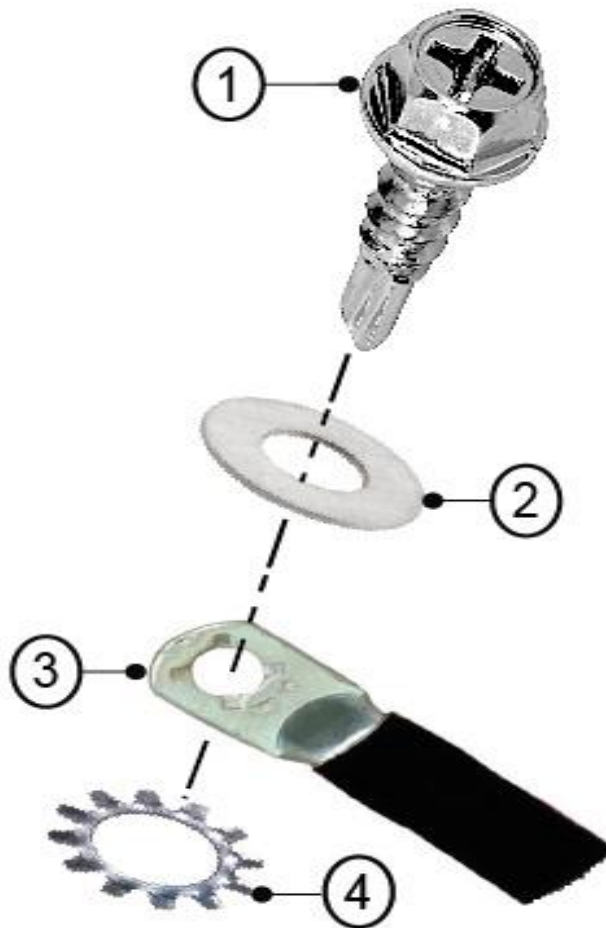
Figure 6-2. Proper ground connection to the mounting frame of a solar panel
