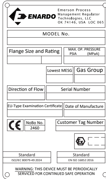
Figure 5. Marking Plate
