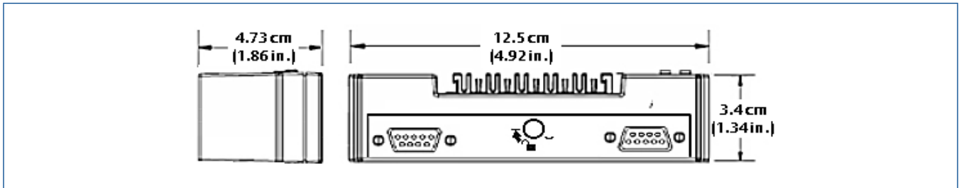
CHARM Baseplate Extender Bottom.
