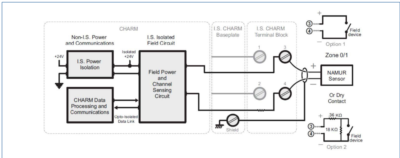
Simplified Circuit and Connection Diagram for LS IS DI NAMUR CHARM.
