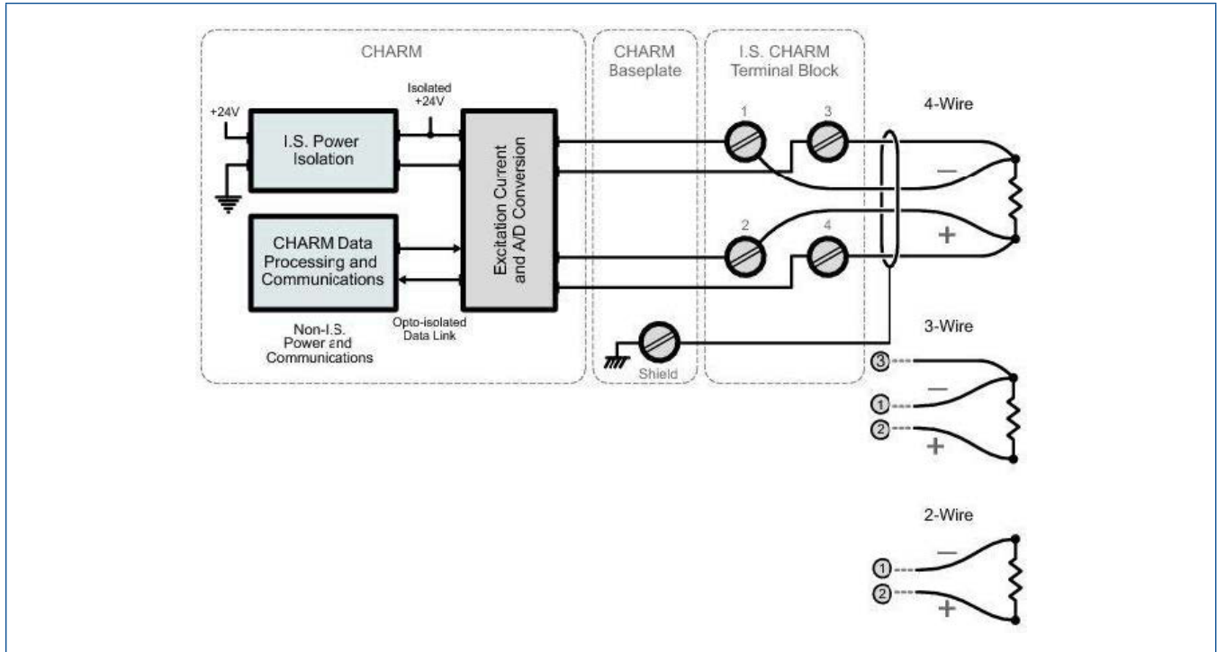
Simplified Circuit and Connection Diagrams for LS IS RTD CHARM.
