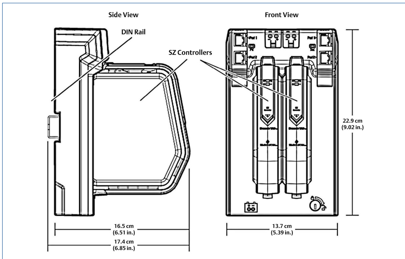
SZ Controller shown on Dual Horizontal Safety Carrier.
