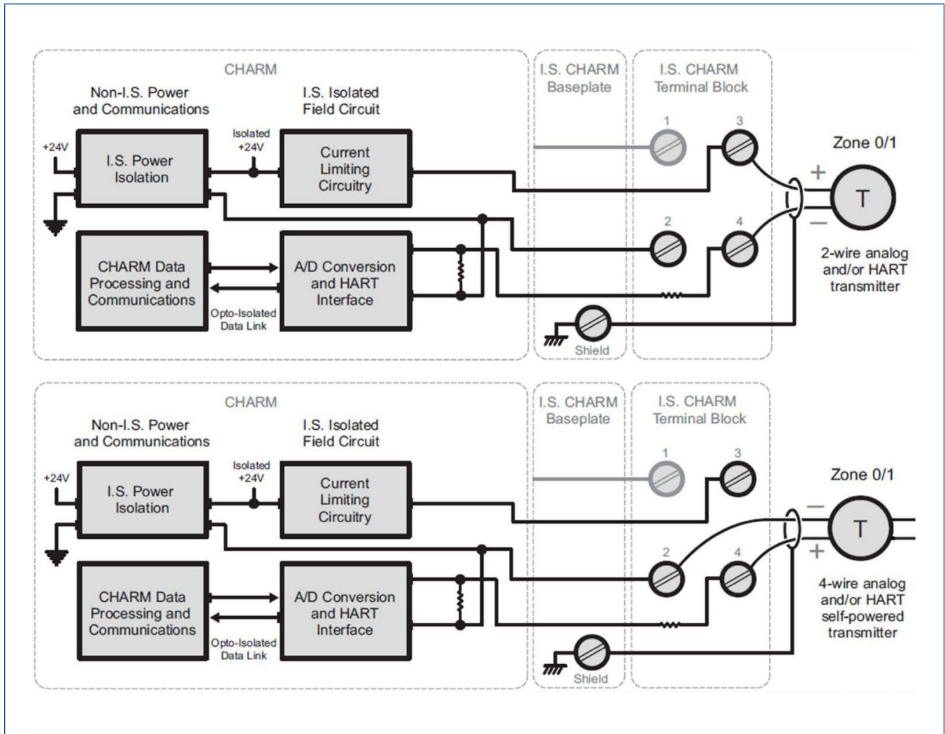
Simplified Circuit and Connection Diagrams for LS IS AI-CHARM 4 to 20 mA HART Two-Wire and Four-Wire transmitters.
