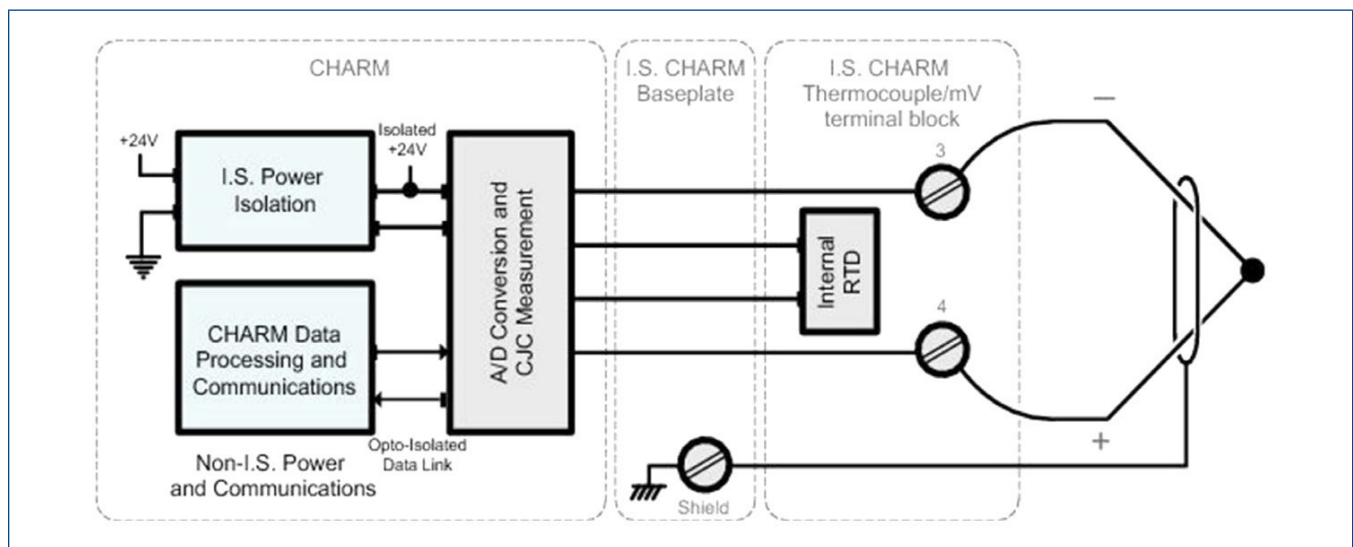
Simplified Circuit and Connection Diagram for LS IS Thermocouple/mV CHARM with IS Thermocouple/mV Terminal Block.
