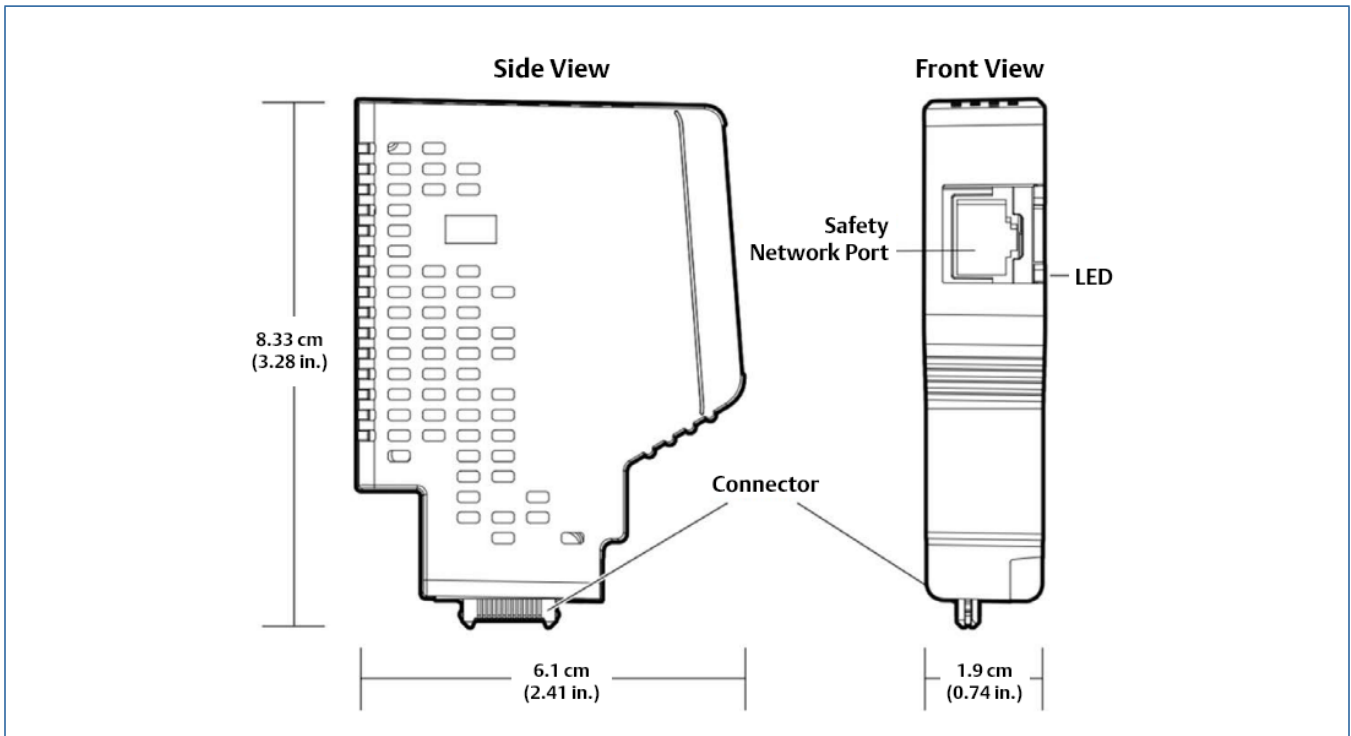
CSLS Safety Network Port.
