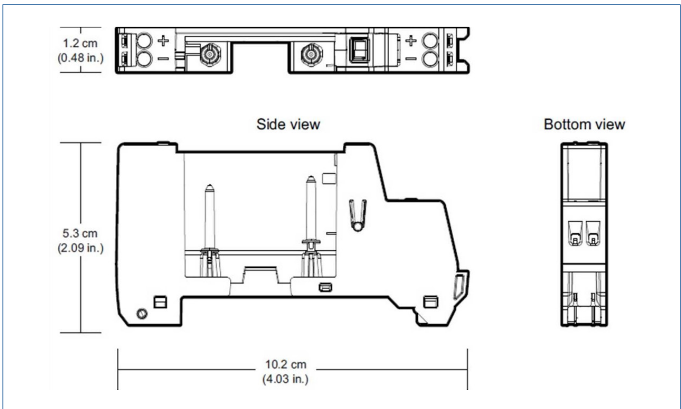
Address Plug Terminal Block for IS Baseplate.
