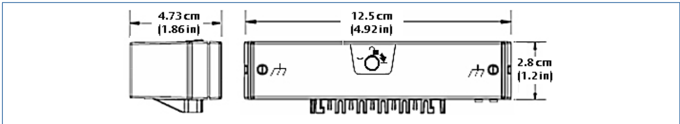
CHARM Baseplate Terminator Top.
