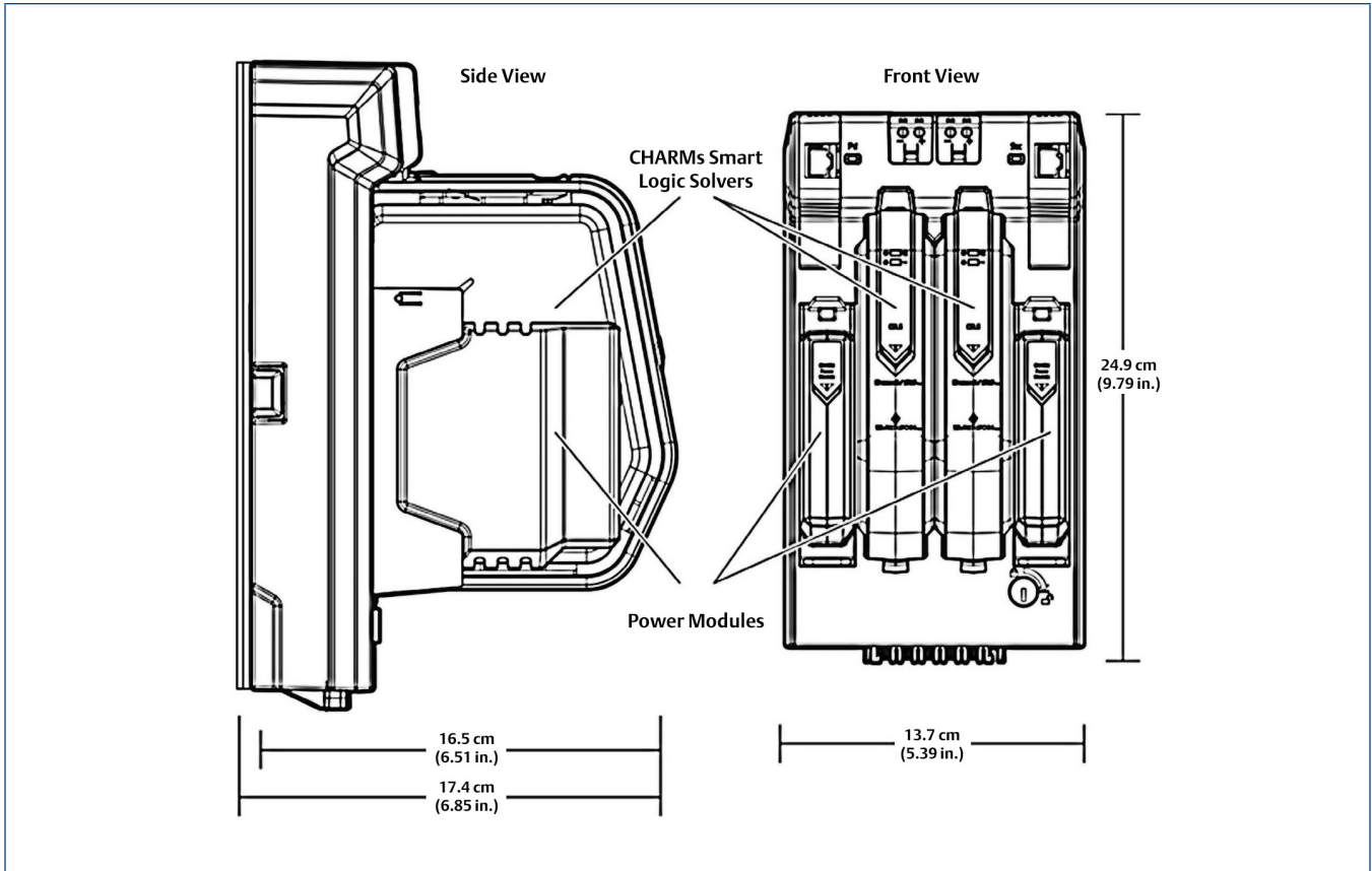
CSLS shown on CSLS Carrier.
