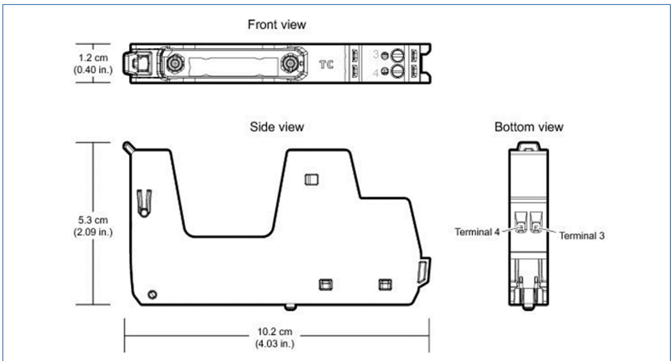
IS CHARM Thermocouple / mV Terminal Block.
