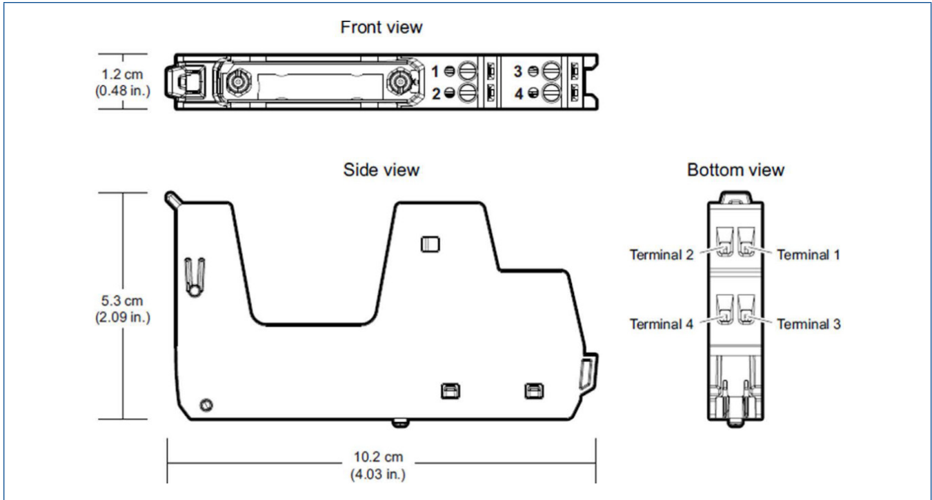
IS CHARM Terminal Block.
