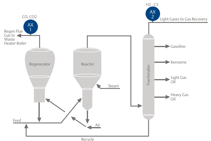
Figure 1 - Flow Diagram of a Typical Fluid Catalytic Cracking Unit
