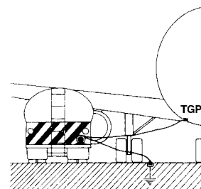
GROUNDING REEL INSTALLED ON A TRUCK. ALLIGATOR CLIP ATTACHES TO TGP GROUNDING STUD, WHICH IS PERMANENTLY INSTALLED ON THE AIRCRAFT. THE OTHER ALLIGATOR CLIP ATTACHES TO GROUND.
