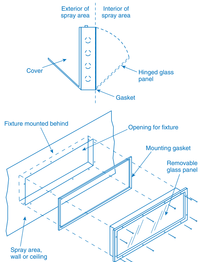
Figure 516.4(C)(3) Example of a Luminaire that is an Integral Part of the Spray Area and is Serviced from Inside the Spray Area. [33:Figure 6.6.3]
