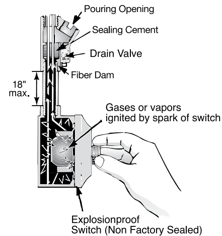
SEALS REQUIRED IN EACH CONDUIT WITHIN 18" OF ARC-PRODUCING DEVICE.
